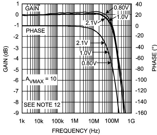
Frequency Response for Various V_G ( A_{VMAX} = 10 )
