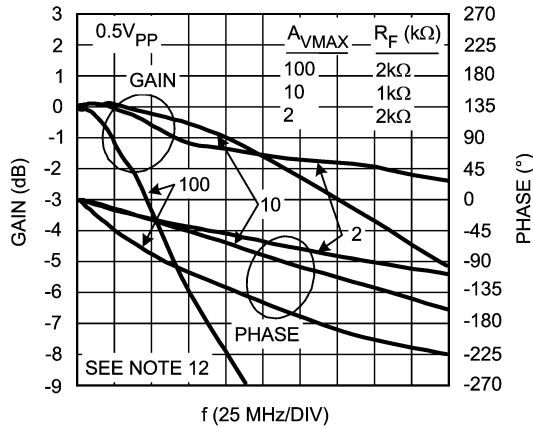
Small Signal Frequency Response for Various A_{VMAX}
