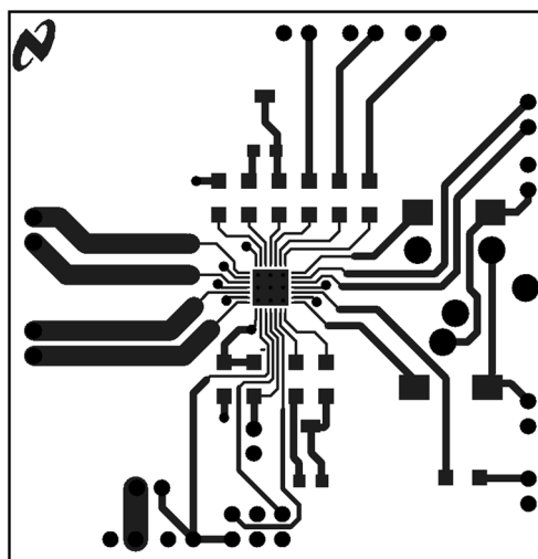
Recommended SP PCB Layout: Top Layer
