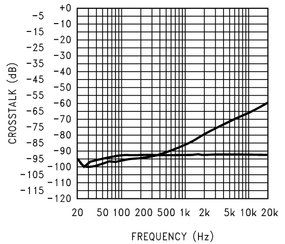
Crosstalk vs Frequency
