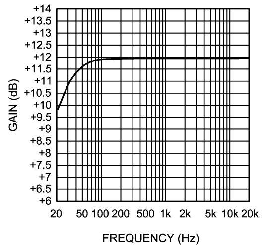
Frequency vs Response
