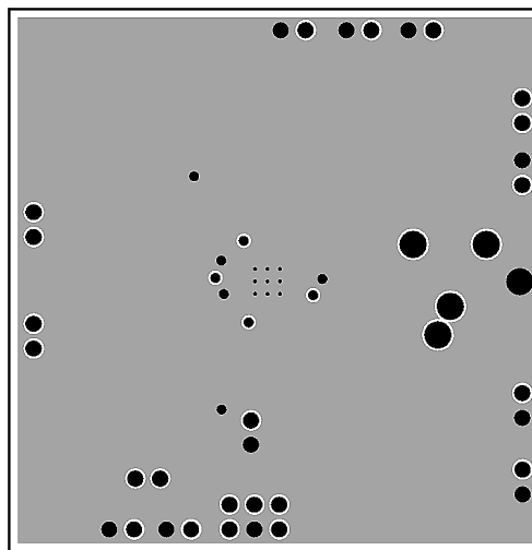
Recommended SP PCB Layout: Bottom Layer
