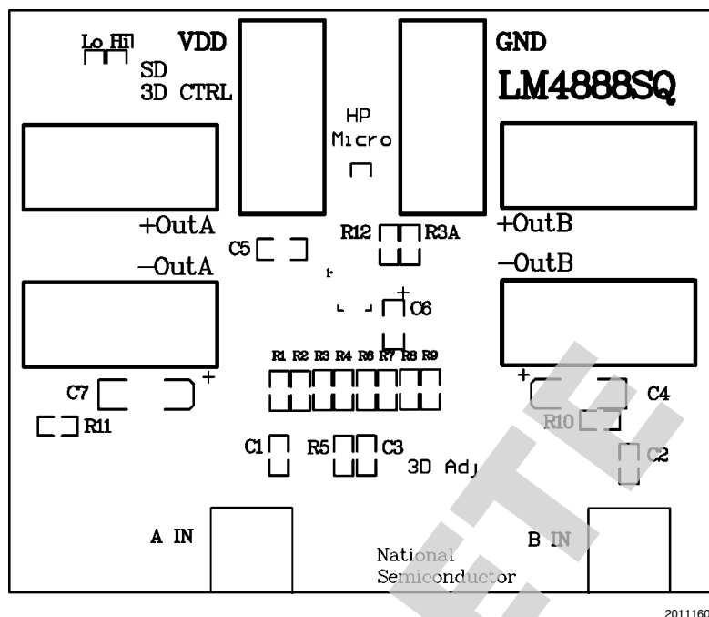
FIGURE 3. Silkscreen
