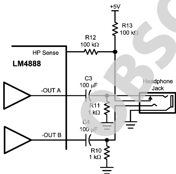
FIGURE 2. Headphone Circuit
