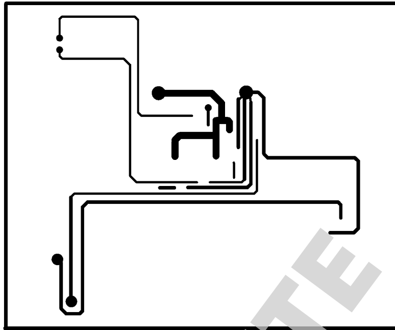
FIGURE 5. Mid layer
