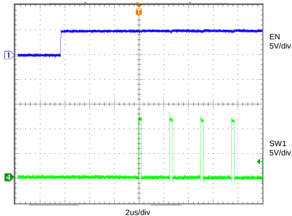
Figure 31 ENABLE Control, 0A
