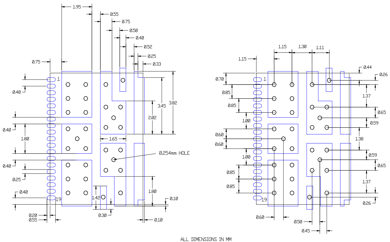
Figure 35: Solder resist
