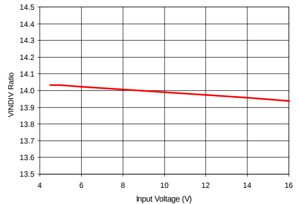
Figure 33 VINDIV to VIN Ratio
