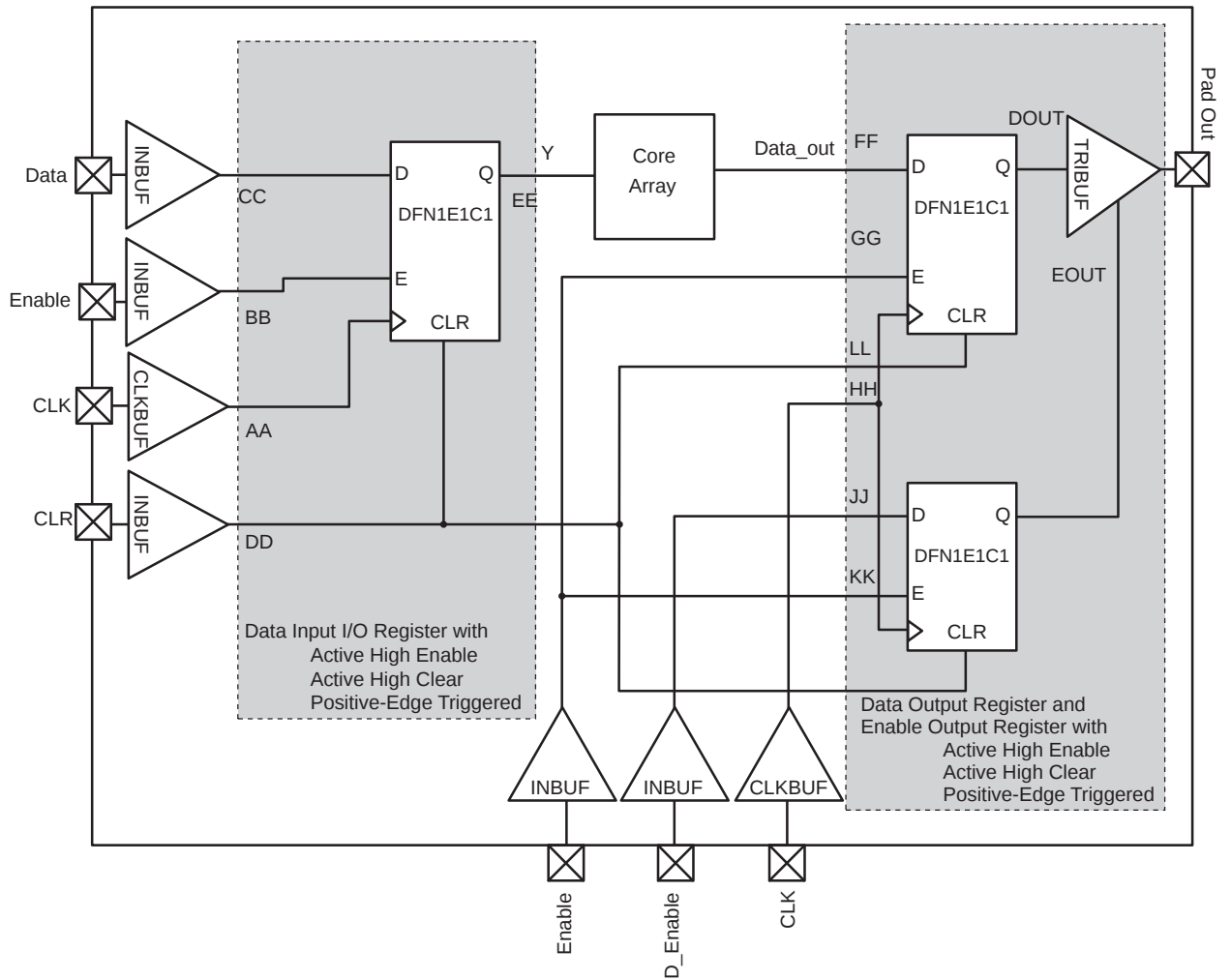
Figure 2-28 • Timing Model of the Registered I/O Buffers with Synchronous Enable and Asynchronous Clear
