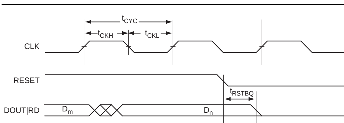
Figure 2-47 • RAM Reset. Applicable to Both RAM4K9 and RAM512×18.
