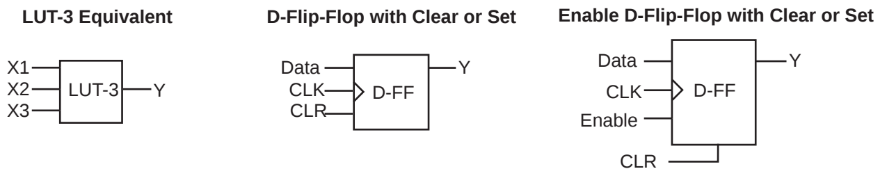
Figure 1-3 • VersaTile Configurations
