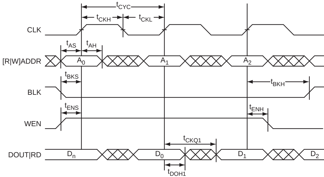
Figure 2-43 • RAM Read for Pass-Through Output. Applicable to Both RAM4K9 and RAM512×18
