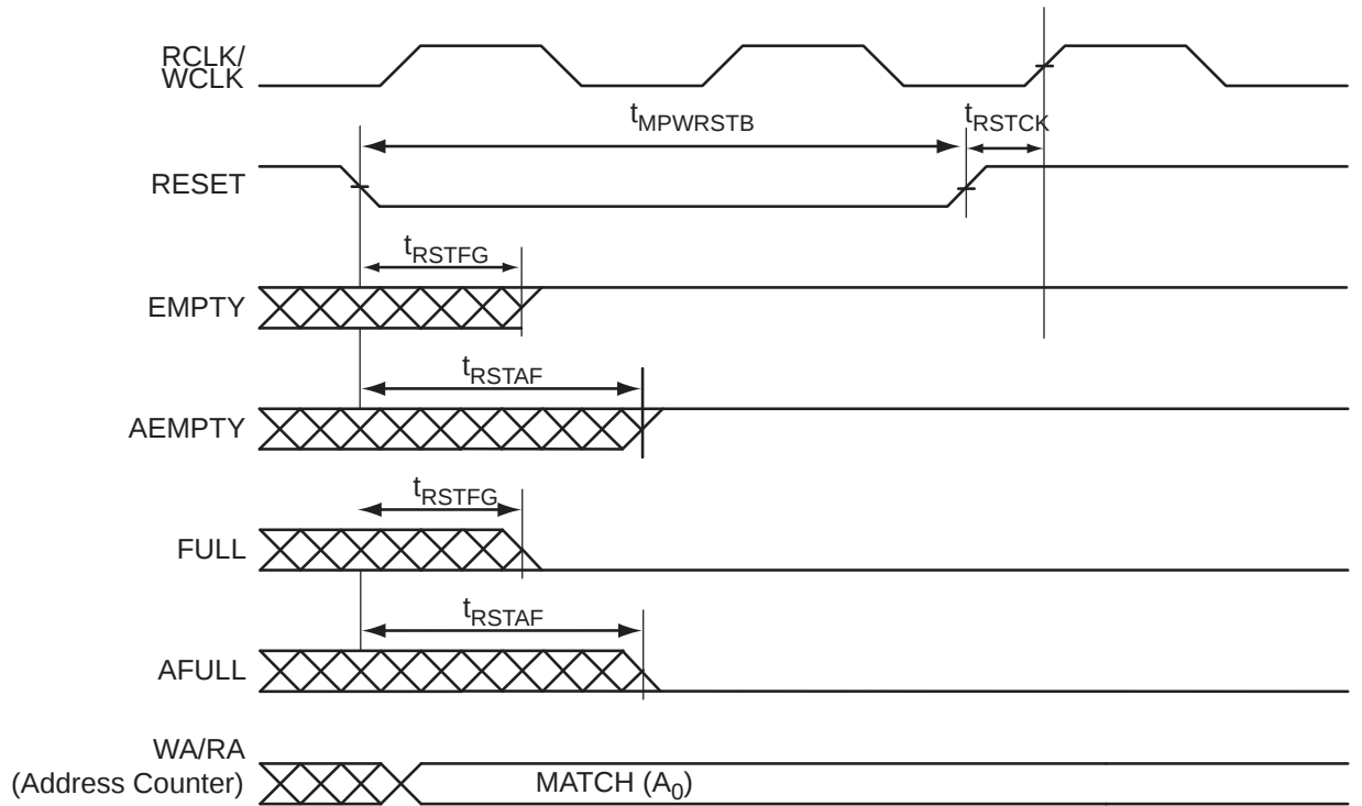
Figure 2-51 • FIFO Reset
