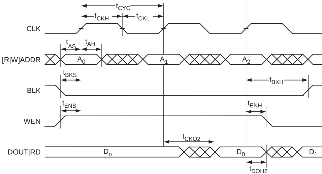
Figure 2-44 • RAM Read for Pipelined Output. Applicable to Both RAM4K9 and RAM512×18
