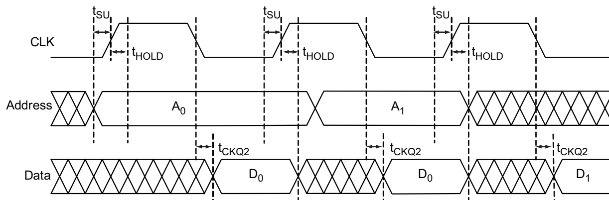
Figure 2-56 • Timing Diagram
