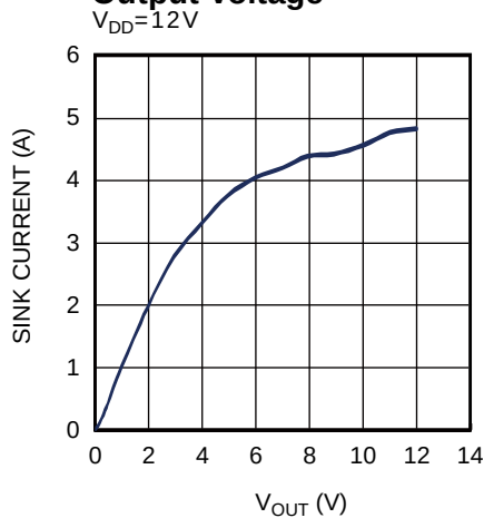
Sink Current vs. Output Voltage V_{DD} = 12V
