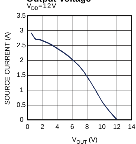
Source Current vs. Output Voltage V_{DD} = 12V
