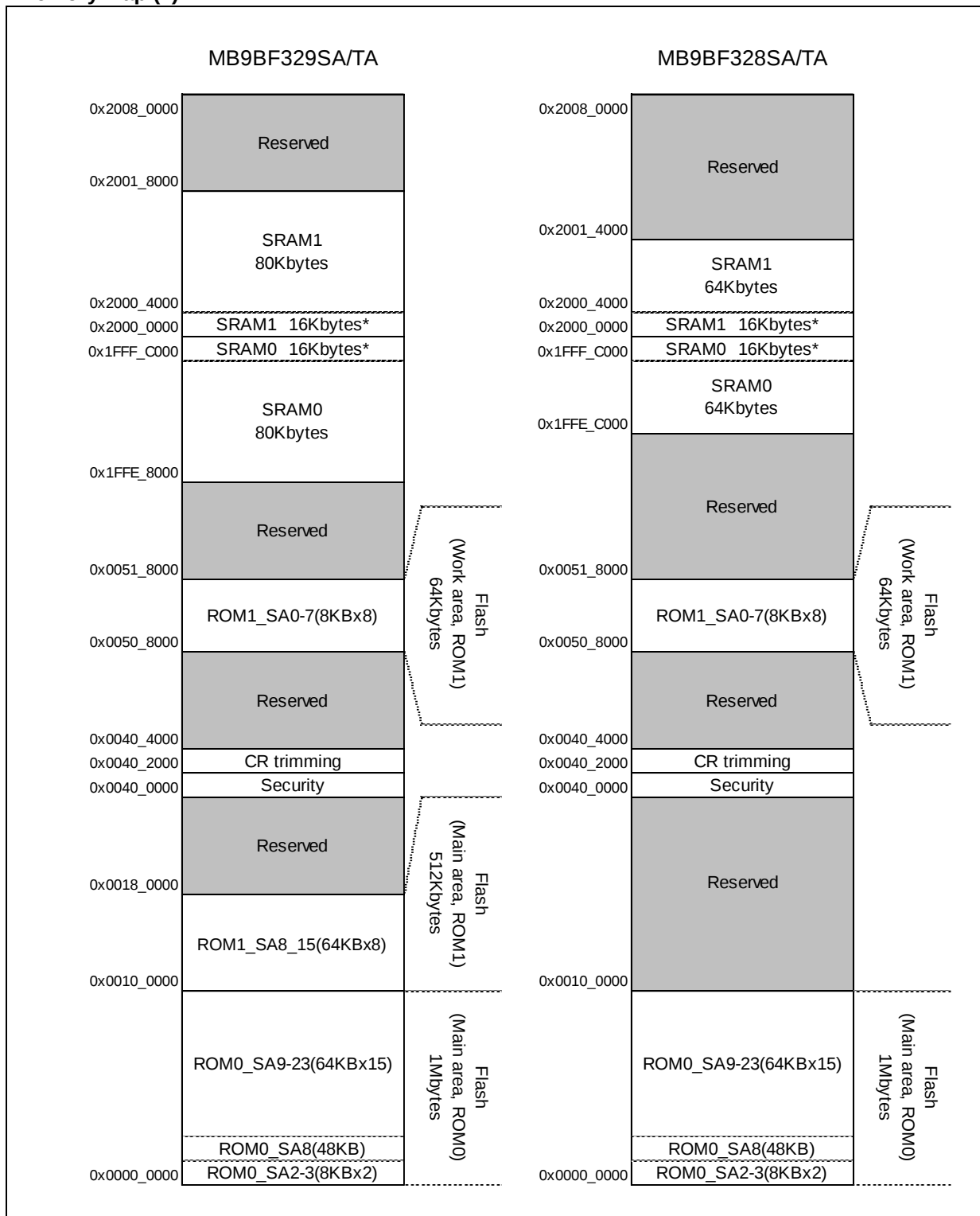
Memory Map (2)
