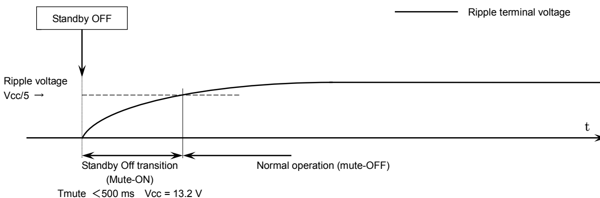
Figure 5 standby-Off Mute
