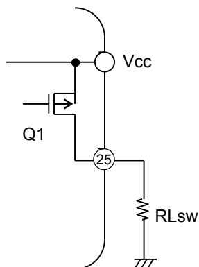
Figure 6 High-side Switch
