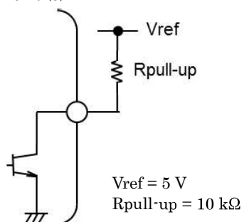
Test circuit (5)
