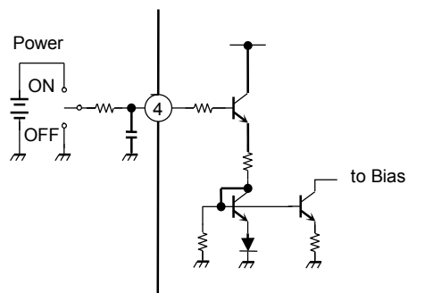
Figure 1 Internal circuit for standby
