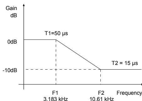
Figure 13. De-Emphasis Curve
