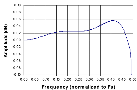
Figure 33. DSM Passband Ripple
