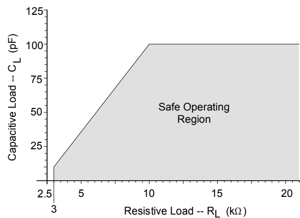
Figure 4. Maximum Loading
