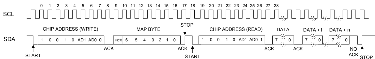
Figure 19. Control Port Timing, I²C Read
