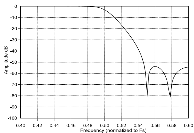
Figure 27. SSM Transition Band
