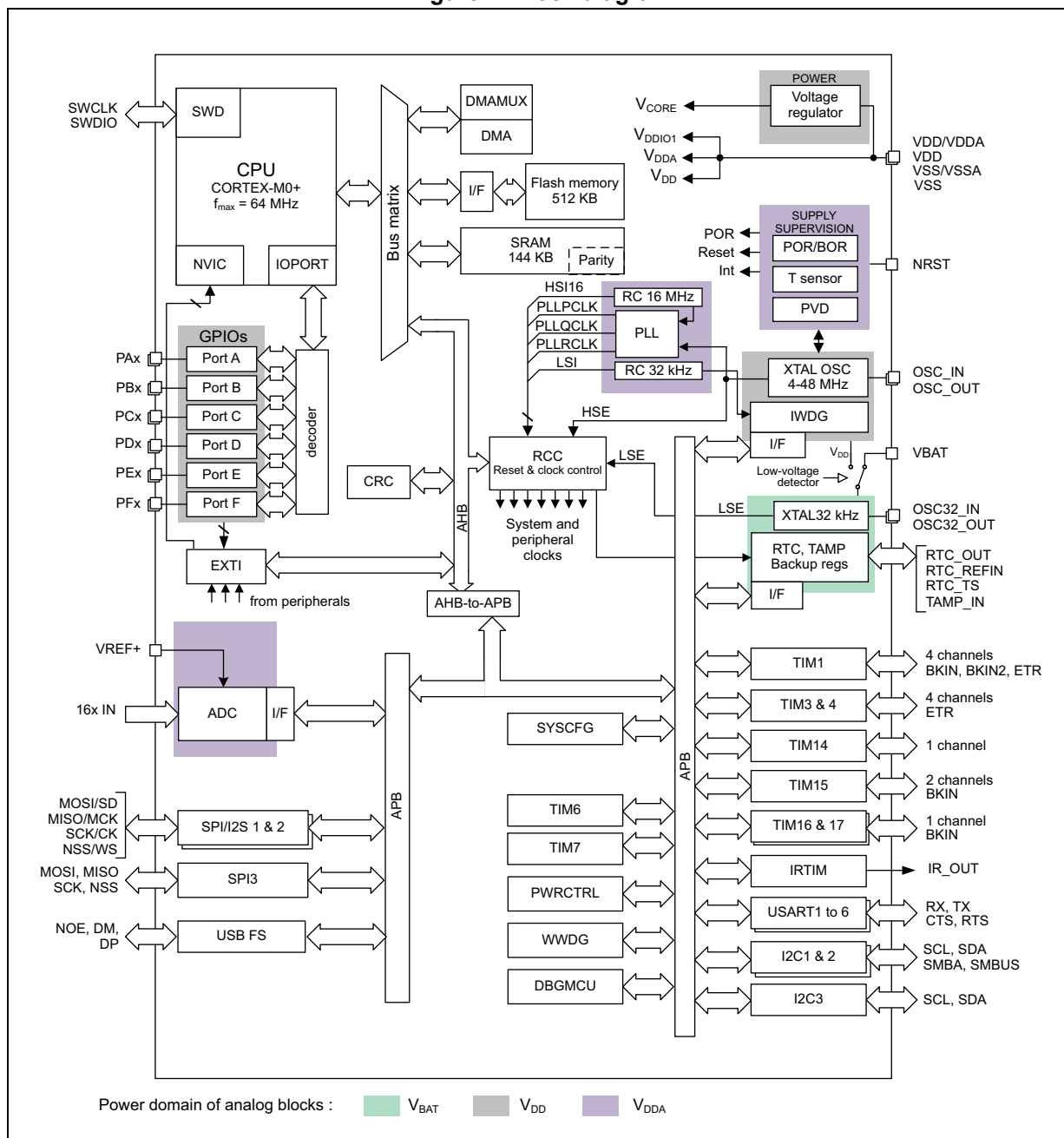
Figure 1. Block diagram
