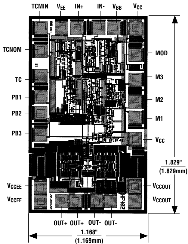
Chip Topography
