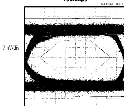
EYE DIAGRAM (OPTICAL) 155Mbps
