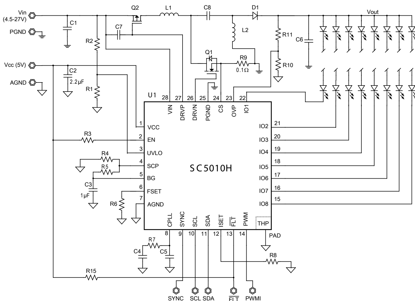
Figure 3 — SEPIC Configuration
