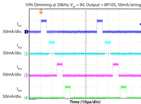
LED Dimming With Phase Shift
