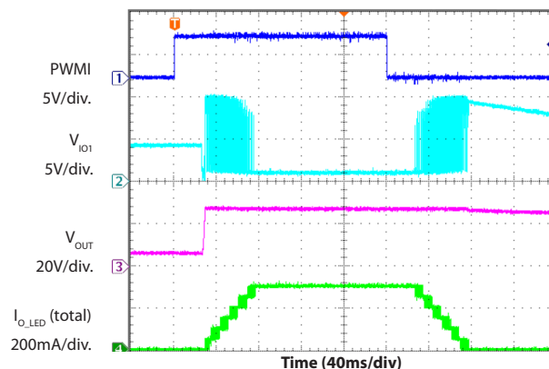
LED Open Circuit Protection
