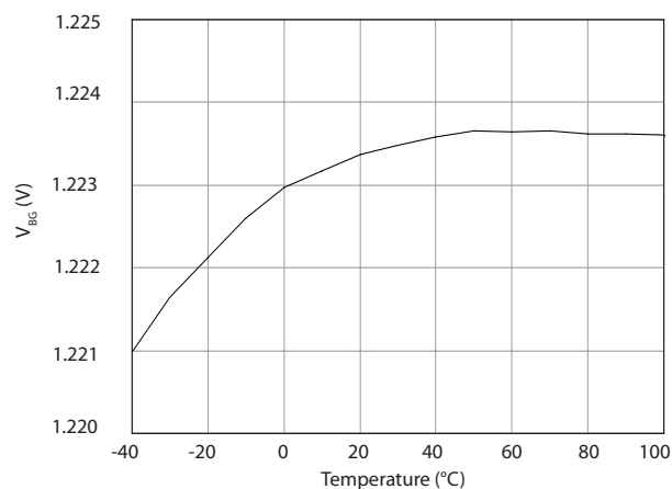
V_{BG} vs. Temperature
