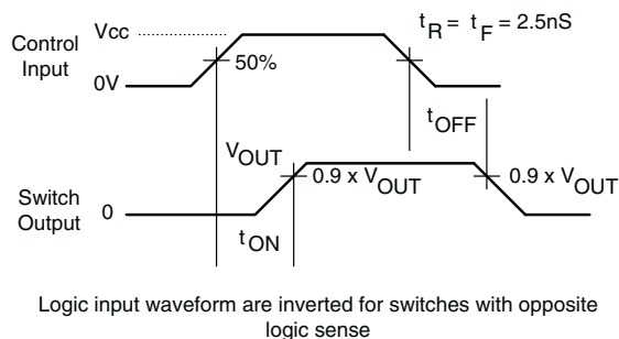
Figure 1. Turn-On/Turn-Off Timing
