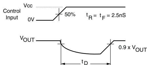
Figure 2. Break-Before-Make Timing`
