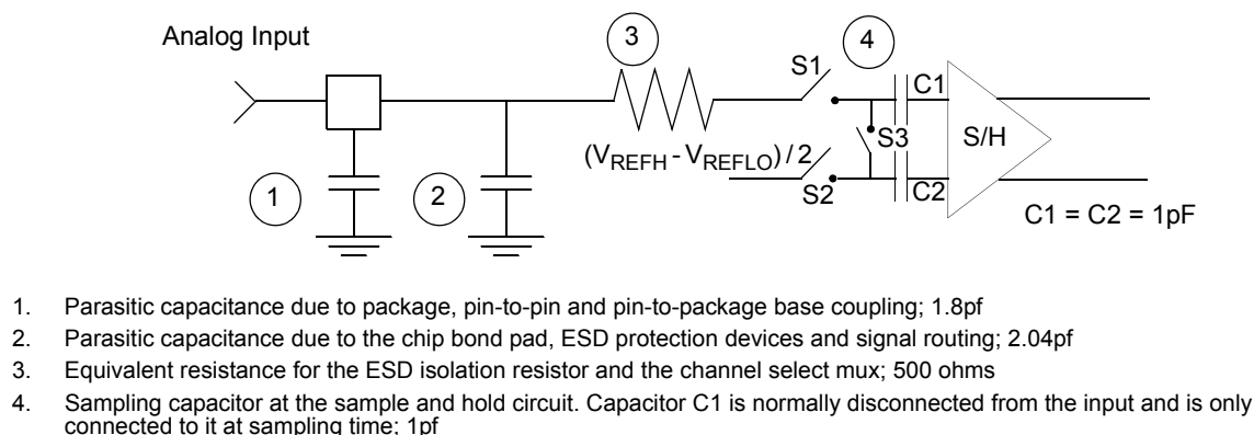
Figure 10-24 Equivalent Circuit for A/D Loading
