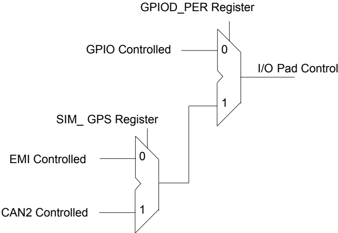
Figure 6-11 Overall Control of GPIOD Pads Using SIM_GPS Control
