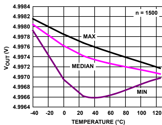
FIGURE 24. V_{OUT} HIGH vs TEMPERATURE, V_S = \pm 2.5V , R_L = 100k
