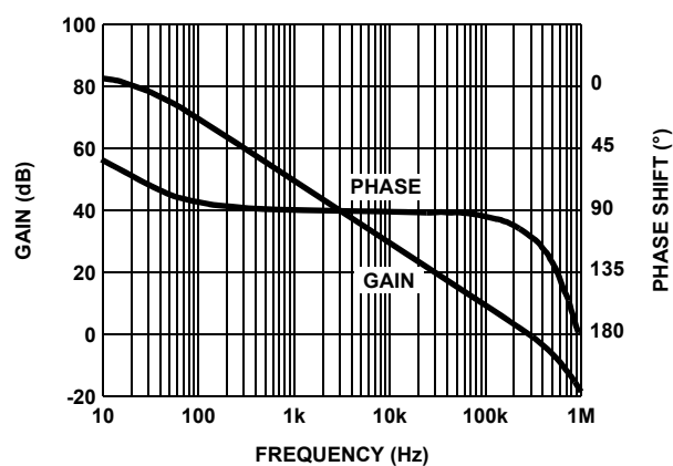
FIGURE 6. OPEN LOOP GAIN AND PHASE vs FREQUENCY ( R_L = 1k\Omega )
