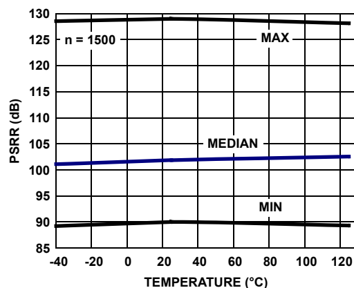
FIGURE 22. PSRR vs TEMPERATURE \pm 1.5V TO \pm 2.5V
