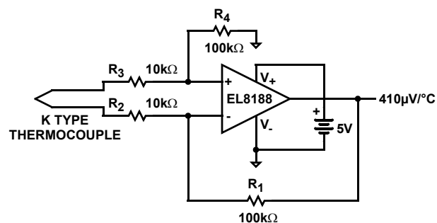
FIGURE 30. THERMOCOUPLE AMPLIFIER
