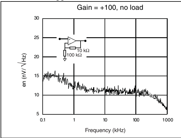
Figure 26. Equivalent input noise voltage ( V_{CC} = \pm 5\text{ V} )
