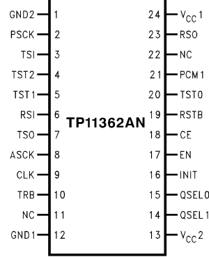
Top View Order Number TP11362AN See NS Package Number N24A
