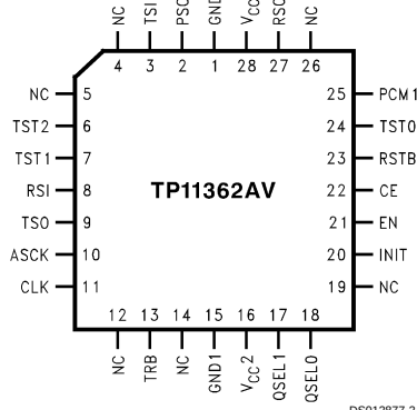
Top View Order Number TP11362AV See NS Package Number V28A
