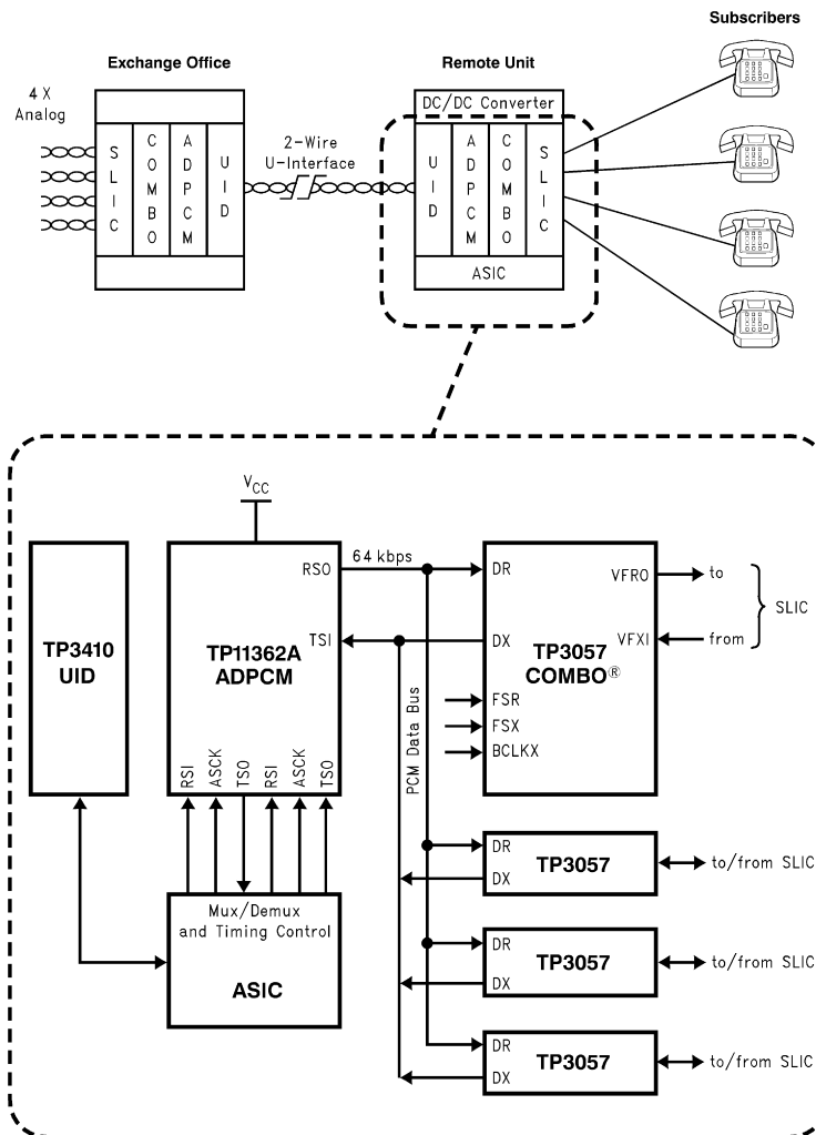
FIGURE 7. Typical Application in an ISDN Pair Gain System
