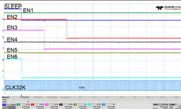
Figure 9-4. Sleep Entry Sequence
