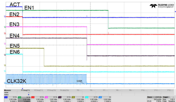
Figure 9-3. Power Down Sequence
