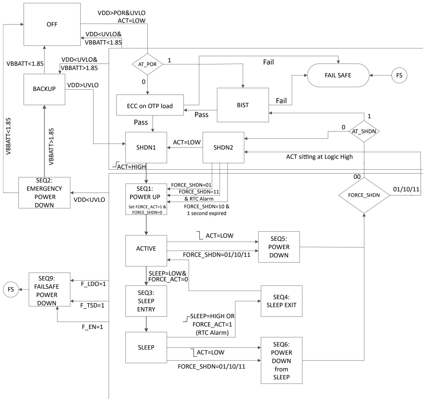
Figure 8-2. TPS38700 State Diagram
