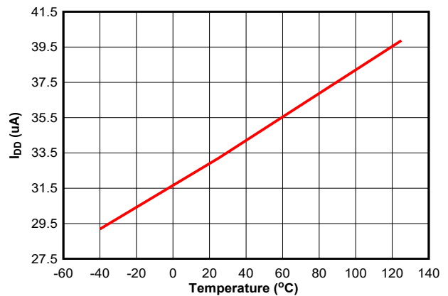
Figure 7-4. I DD Shutdown Current vs. Temperature
