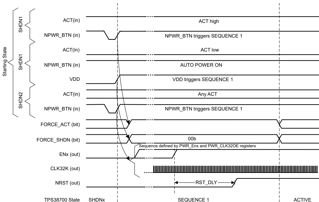
Figure 8-5. Power Up with NPWR_BTN Enabled
