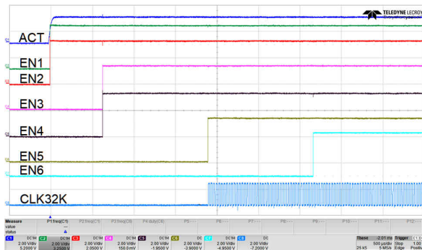
Figure 9-2. Power Up Sequence
