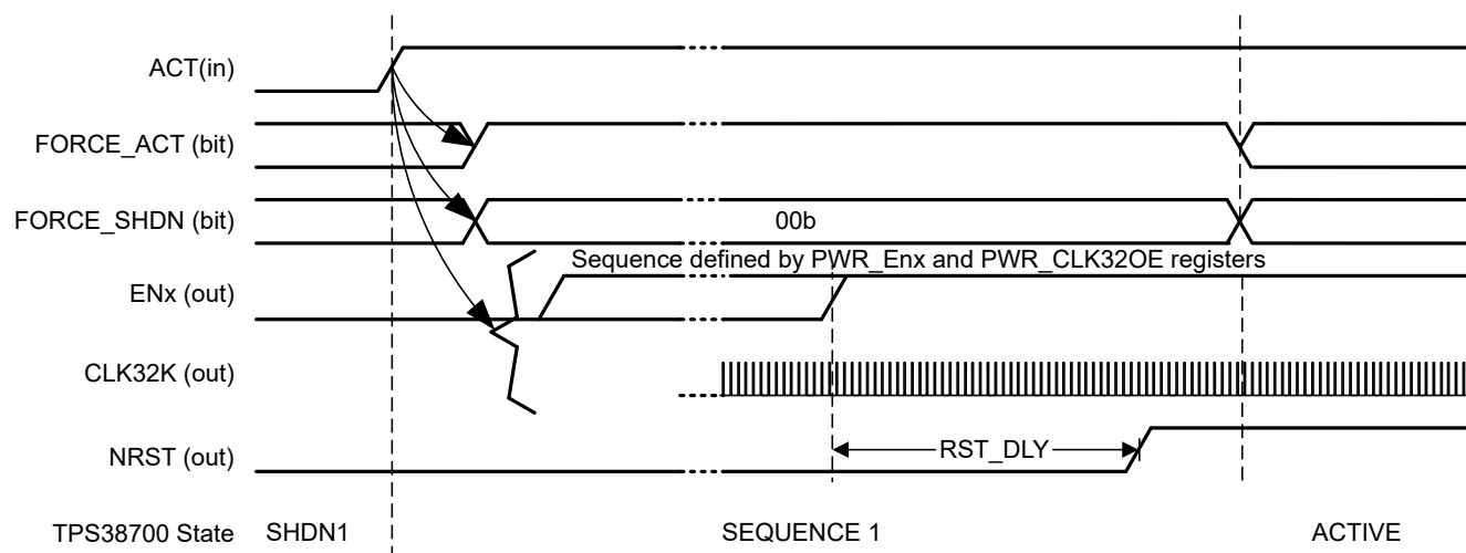
Figure 8-4. Power Up with NPWR_BTN Disabled - ACT controlled
