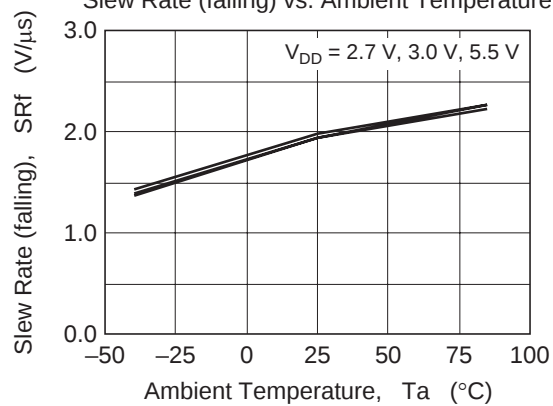
Figure 22 HA1630D08 Slew Rate (falling) vs. Ambient Temperature
