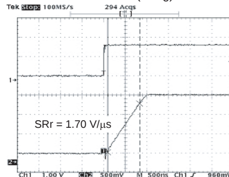
Figure 20 HA1630D08 Slew Rate (rising)
