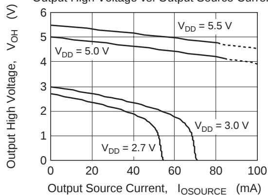
Figure 5 HA1630D08 Output High Voltage vs. Output Source Current
