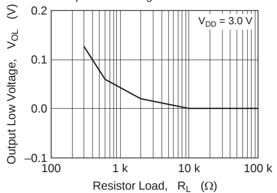
Figure 4 HA1630D08 Output Low Voltage vs. Resistor Load
