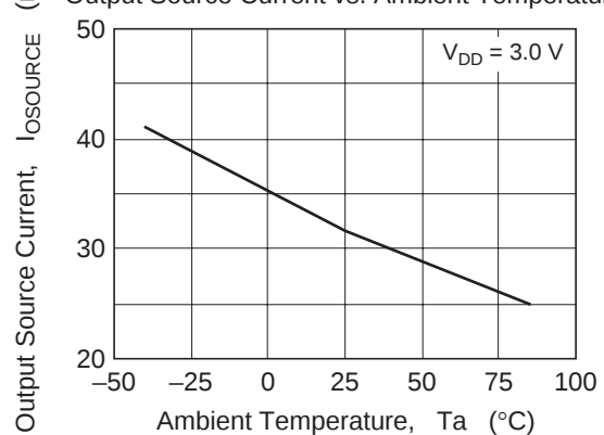
Figure 6 HA1630D08 Output Source Current vs. Ambient Temperature
