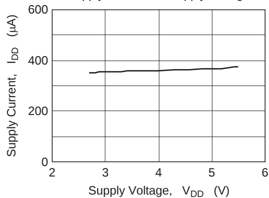
Figure 1 HA1630D08 Supply Current vs. Supply Voltage
