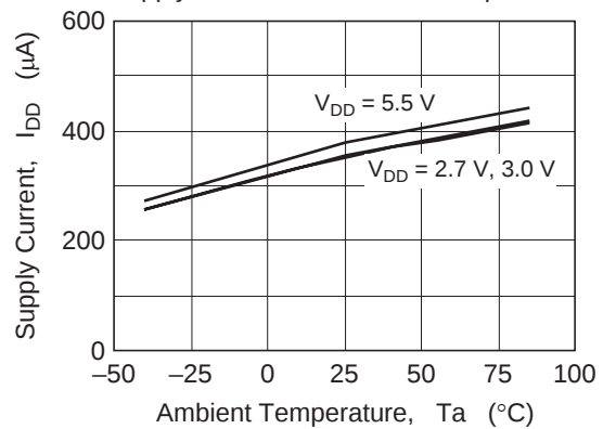
Figure 2 HA1630D08 Supply Current vs. Ambient Temperature
