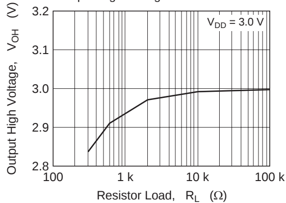
Figure 3 HA1630D08 Output High Voltage vs. Resistor Load
