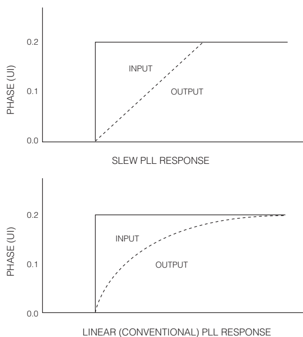
Fig. 16 PLL Characteristics
