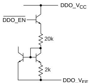
Fig. 14 \overline{\text{DDO\_EN}} Circuit
