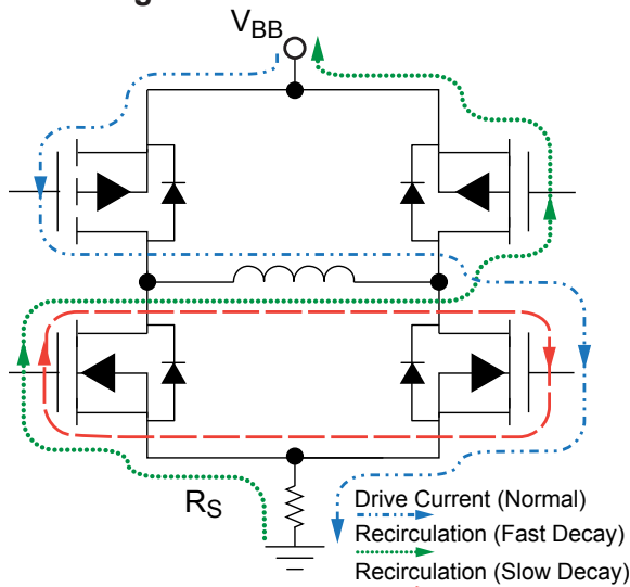
Figure 1 — Load-Current Paths
