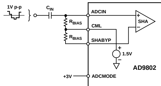
Figure 23. AC-Coupled Input
