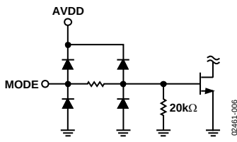
Figure 6. Equivalent MODE Input Circuit
