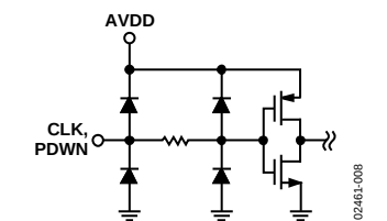
Figure 8. Equivalent Digital Input Circuit
