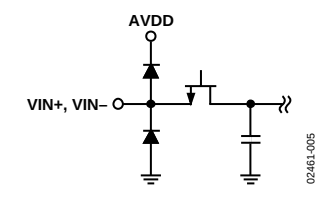
Figure 5. Equivalent Analog Input Circuit
