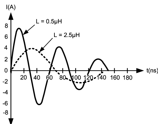
Figure 4. MM Waveform
