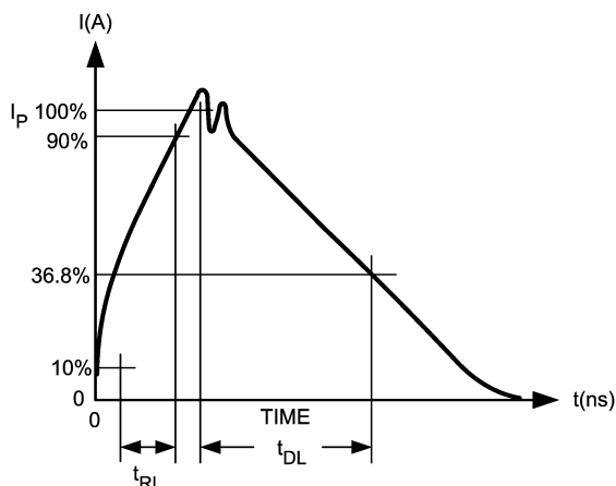
Figure 2. HBM Waveform
