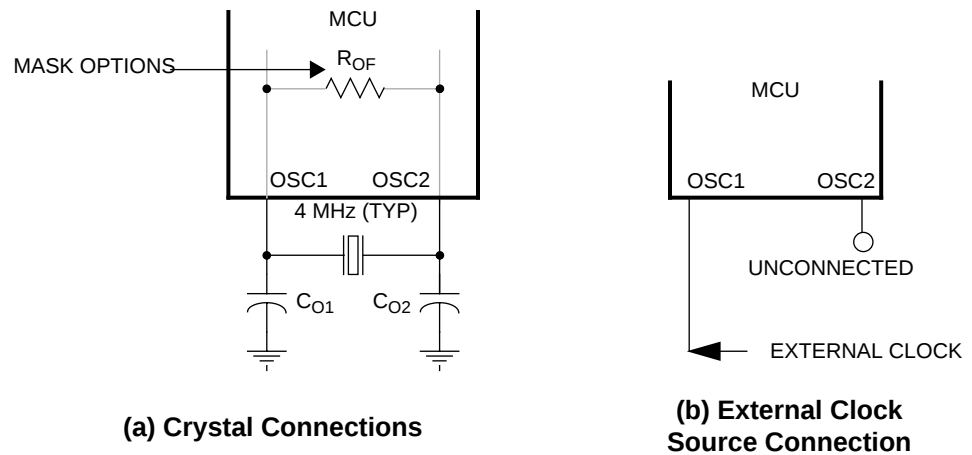
Figure 1-3. Oscillator Connections
