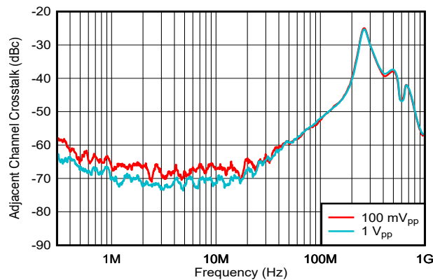
Figure 6-11. Adjacent Channel Crosstalk
