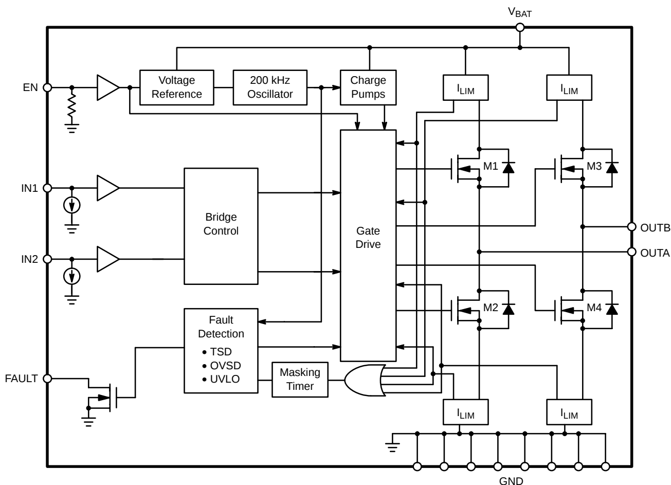
Figure 1. Block Diagram
