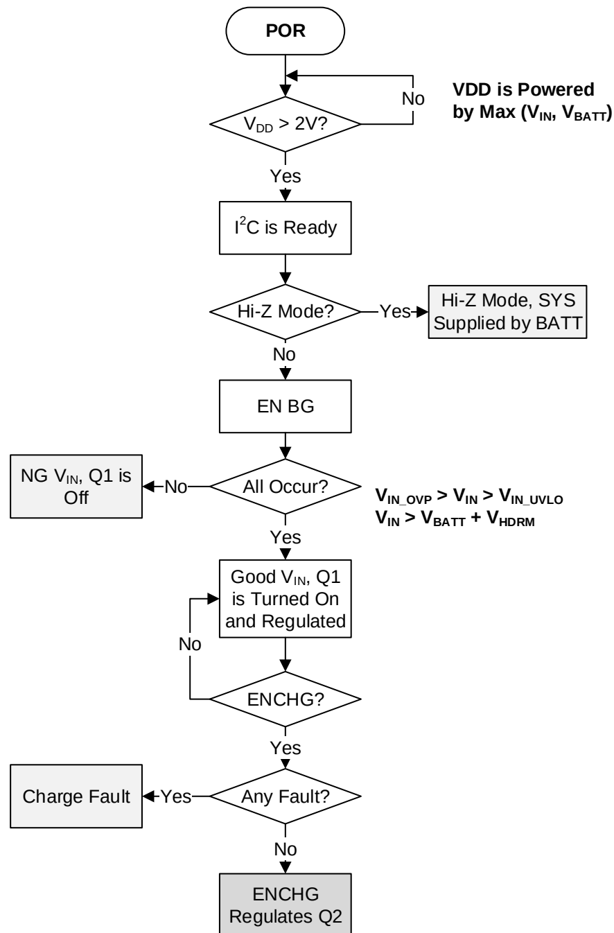
Figure 20: Input Power Start-Up Flowchart
