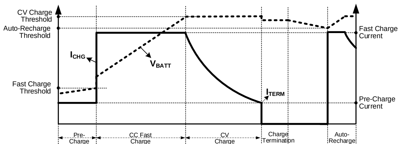
Figure 5: Battery Charge Profile
