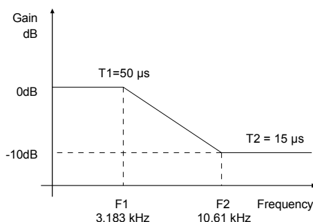
Figure 12. De-Emphasis Curve
