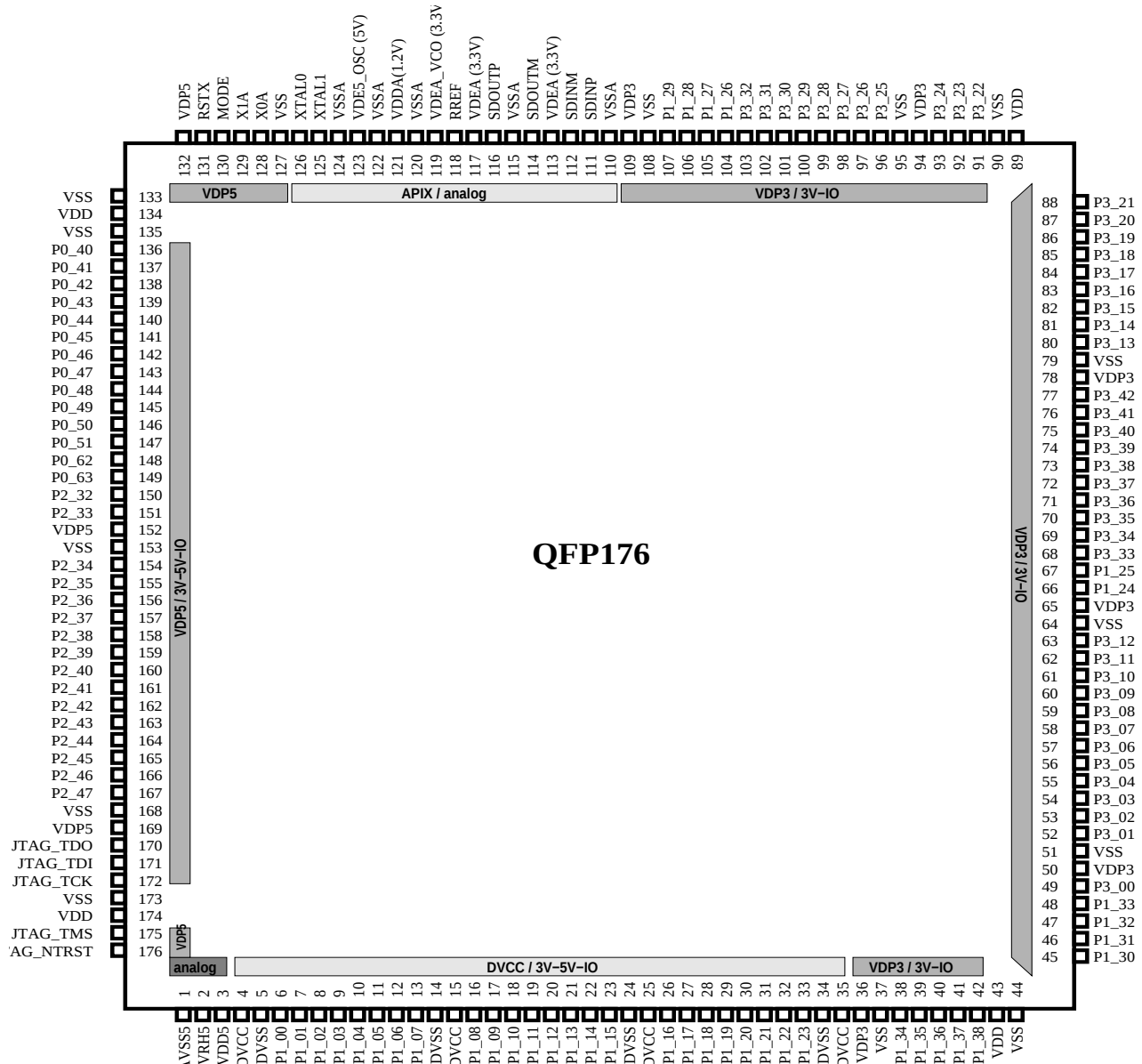
Figure 1. QFP-176 Package
