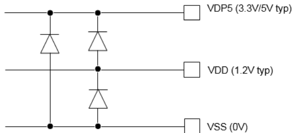
Figure 20. ESD Diodes between VDP5, VDD, and VSS
