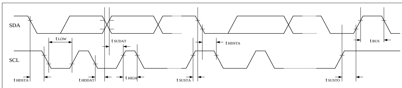
Figure 9. I 2 C Timing
