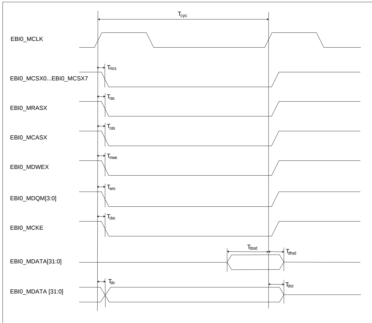
Figure 13. SDRAM Access Timing
