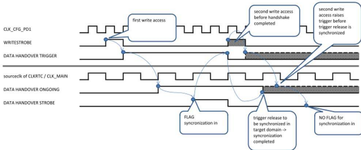
Figure 29. Handshake Synchronization
