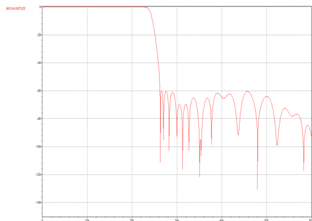
Figure 84 ADC Digital Filter Frequency Response (128OSR)
