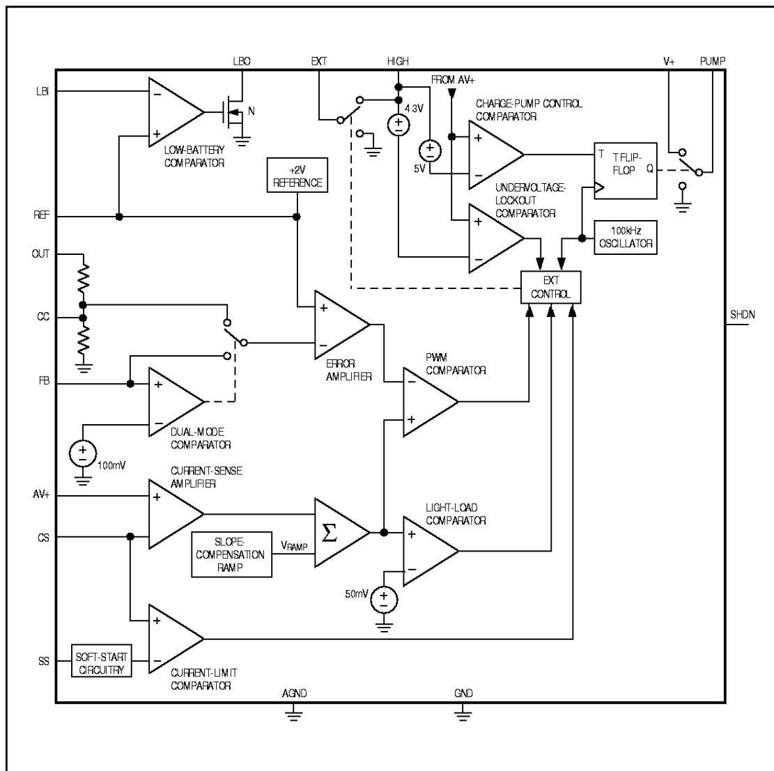
Figure 2. Block Diagram
