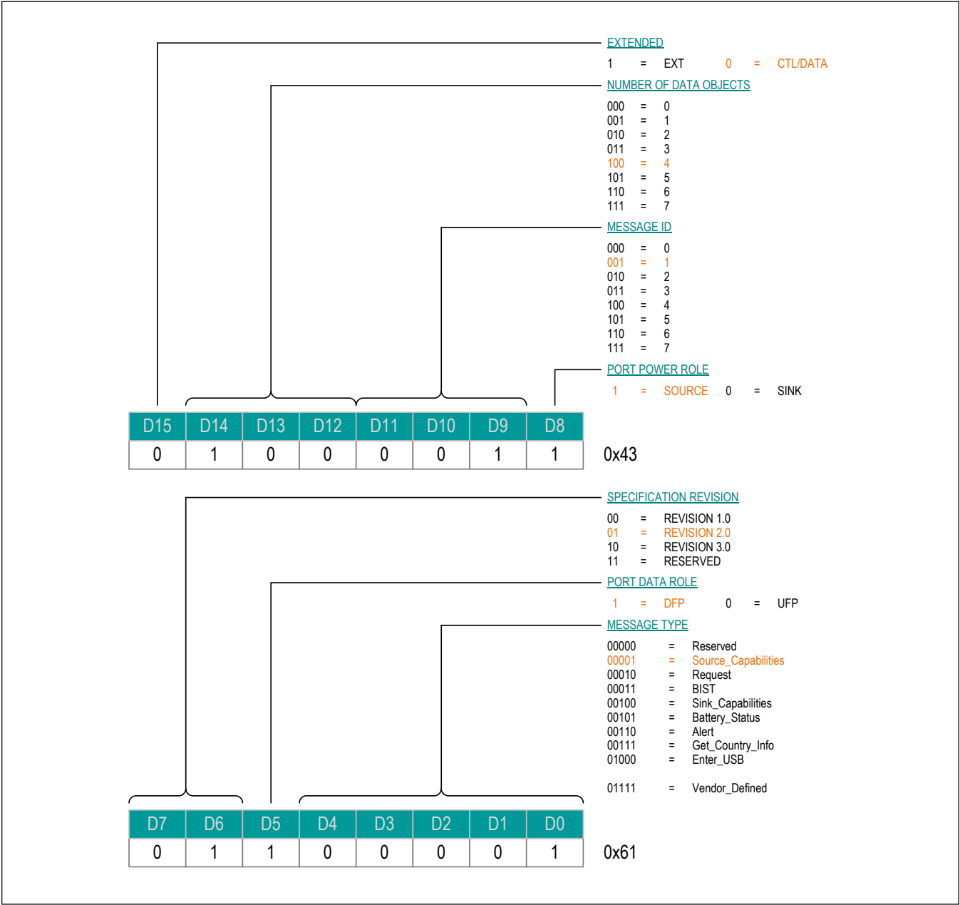
Figure 34. Message Header – "Source_Capabilities"
