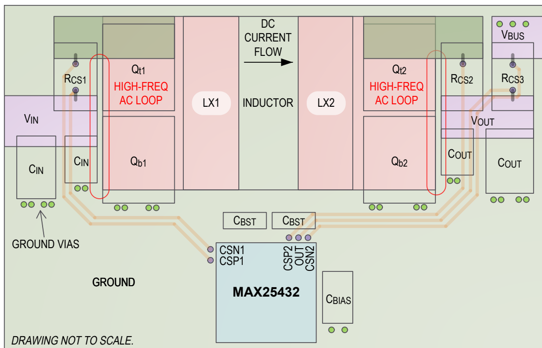
Figure 40. Recommended Buck-Boost PCB Layout
