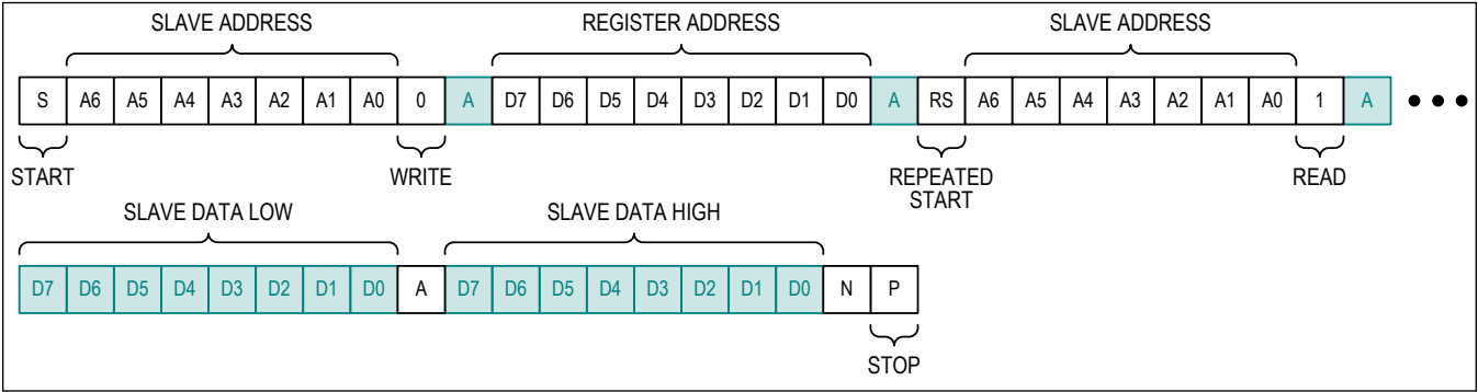
Figure 25. Read Word
