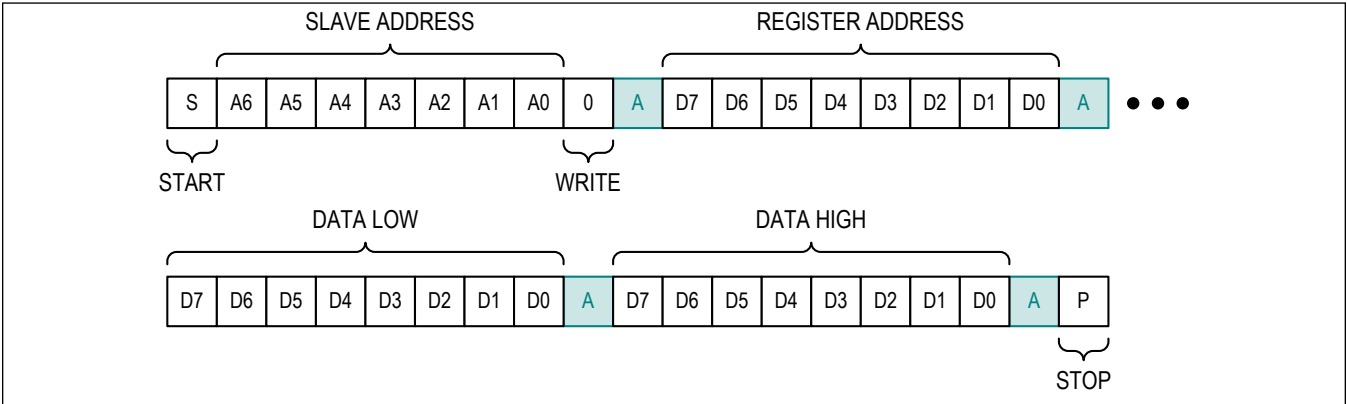
Figure 26. Write Word
