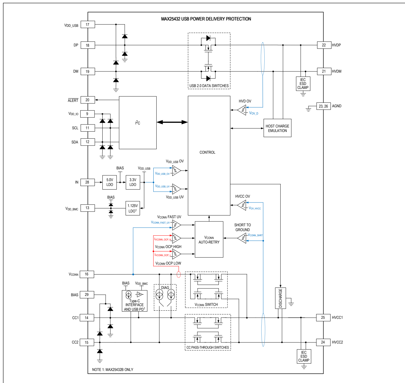
Figure 15. USB Power Delivery Protection Block Diagram
