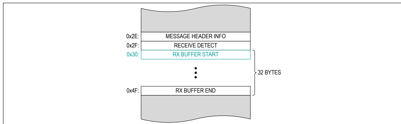
Figure 31. Receive Buffer
