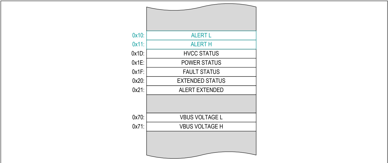
Figure 30. Status Registers
