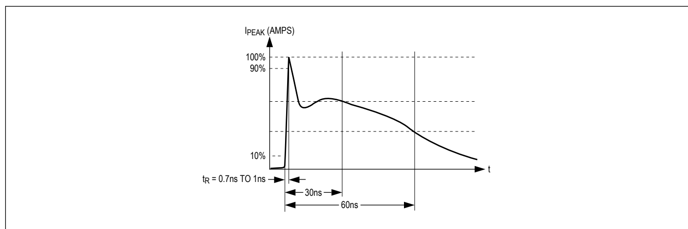
Figure 47. IEC 61000-4-2 Current Waveform
