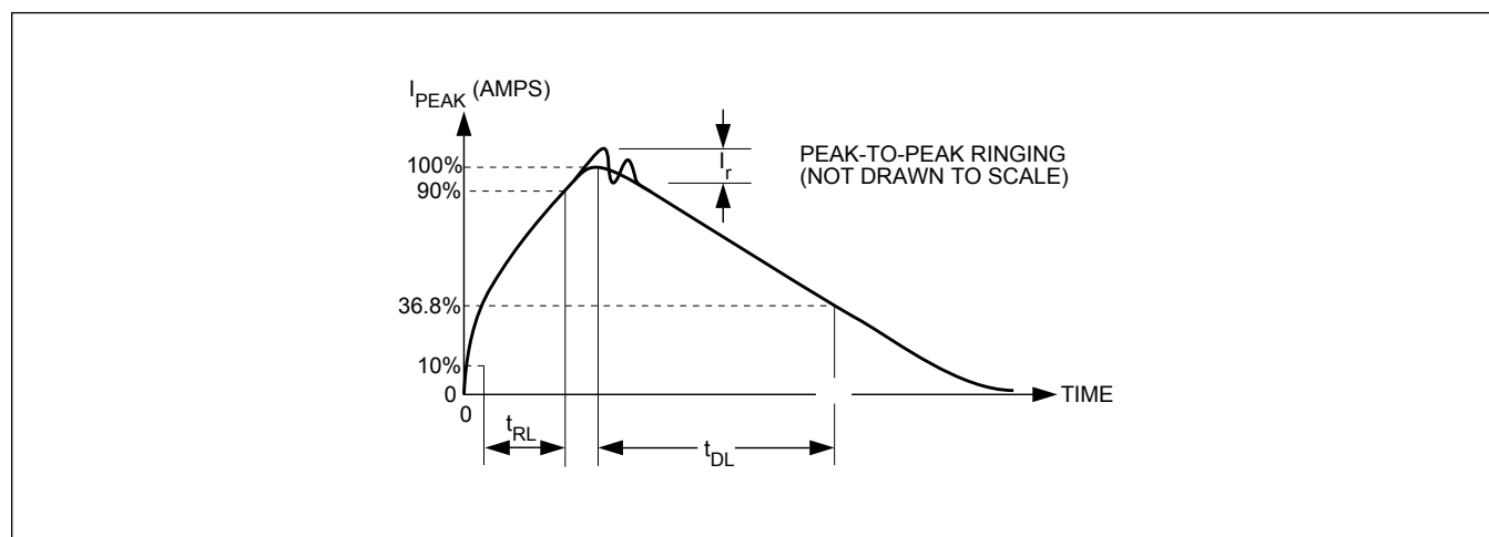
Figure 45. Human Body Current Waveform
