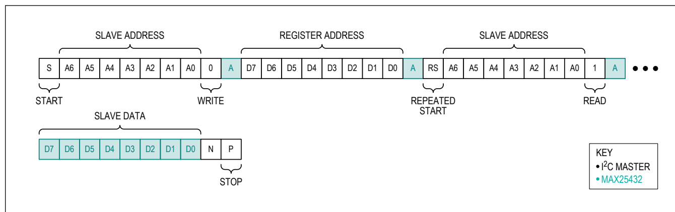
Figure 23. Read Byte
