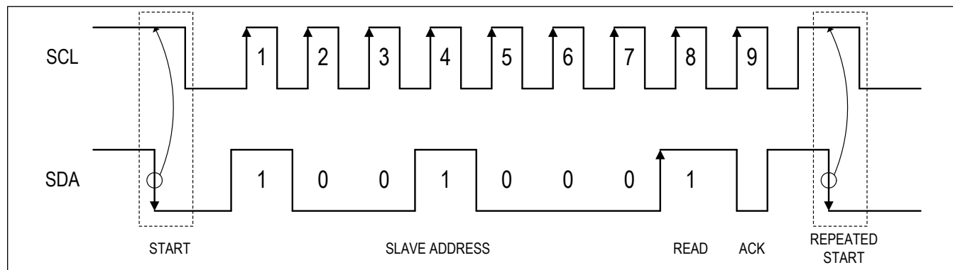
Figure 22. REPEATED START Condition
