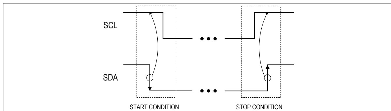
Figure 21. START and STOP Conditions
