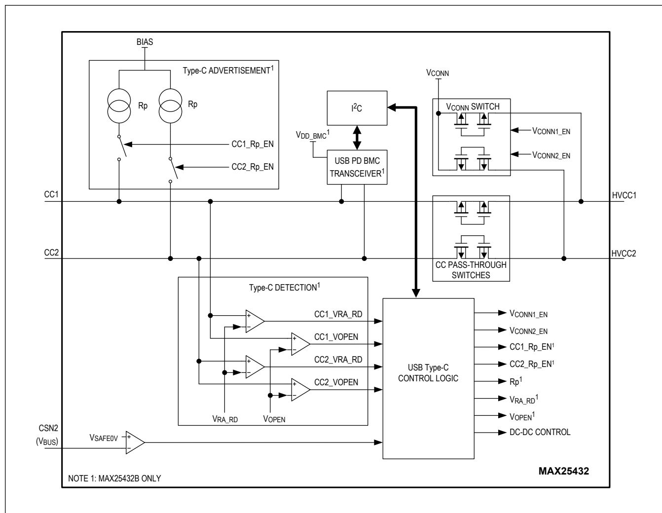
Figure 5. USB Type-C Functional Block Diagram
