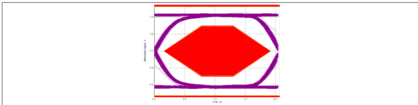
Figure 42. Near-Eye Diagram (with No MAX25432)
