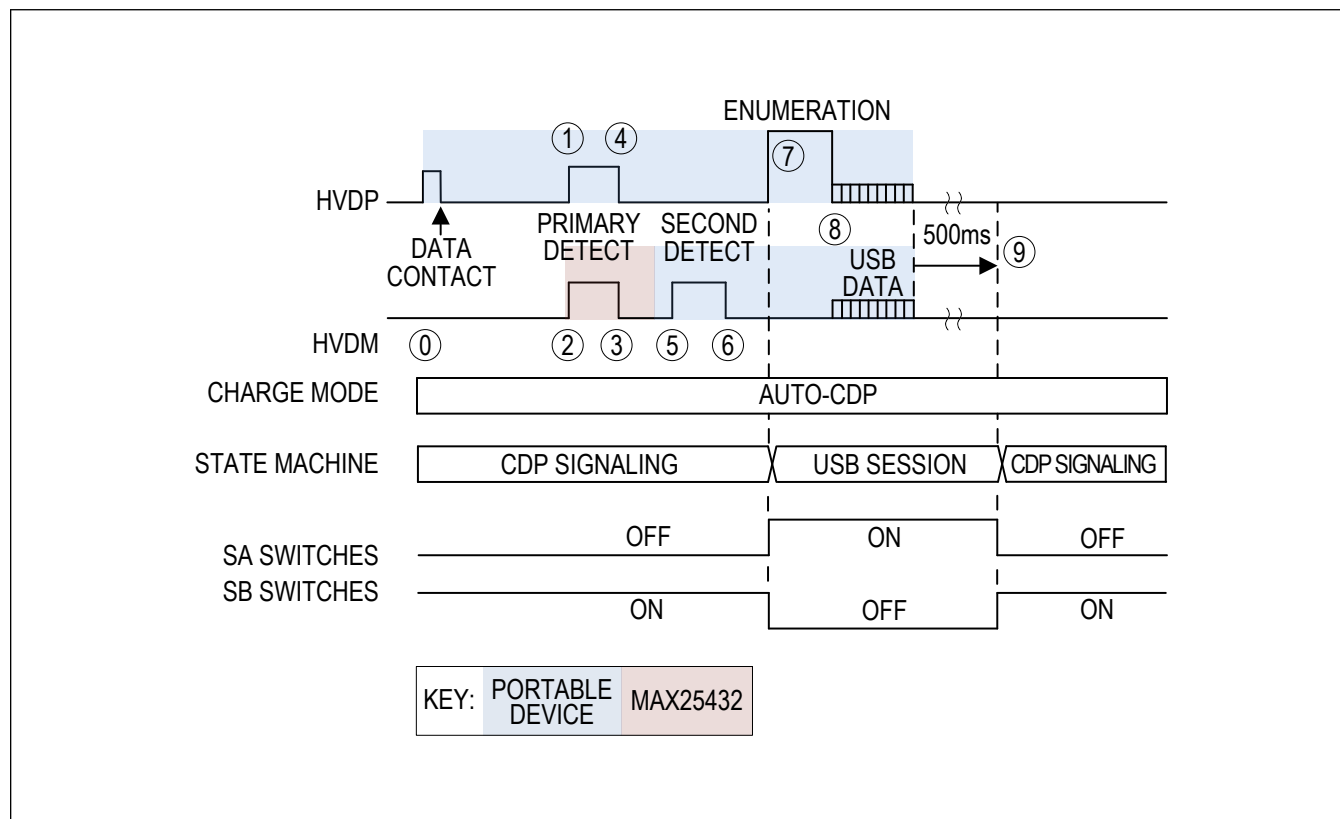
Figure 14. Auto-CDP State Diagram
