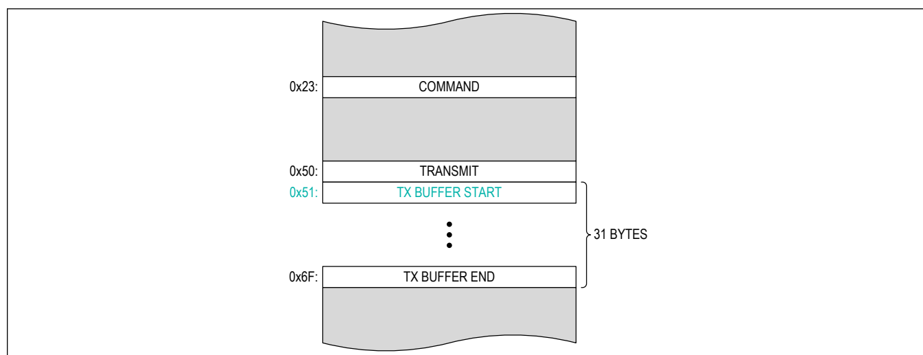
Figure 33. Transmit Buffer
