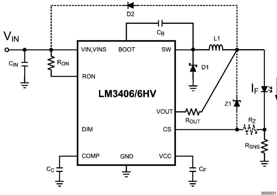
FIGURE 4. Two Methods of Output Open Circuit Protection
