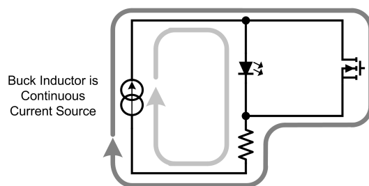
FIGURE 18. Parallel FET Dimming Current Loops
