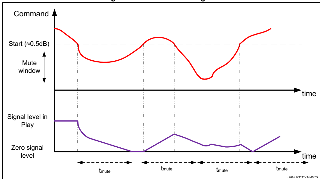
Figure 45. Mixed mute diagram
