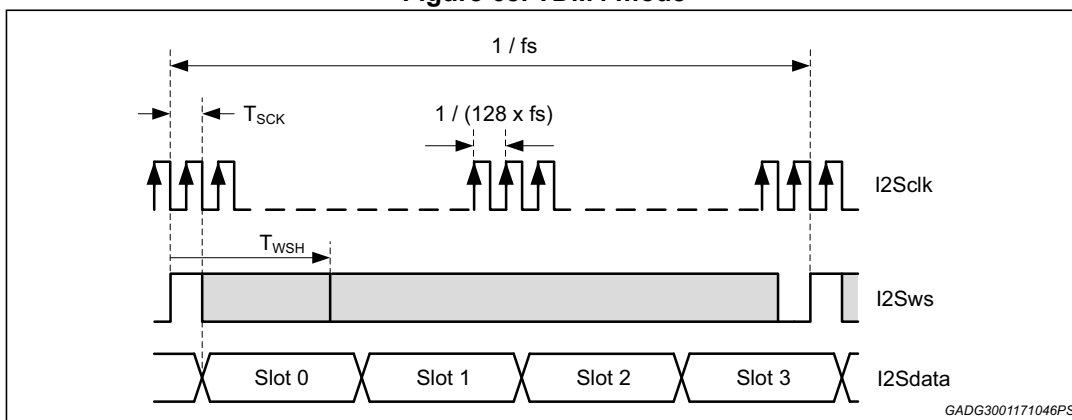
Figure 68. TDM4 mode
