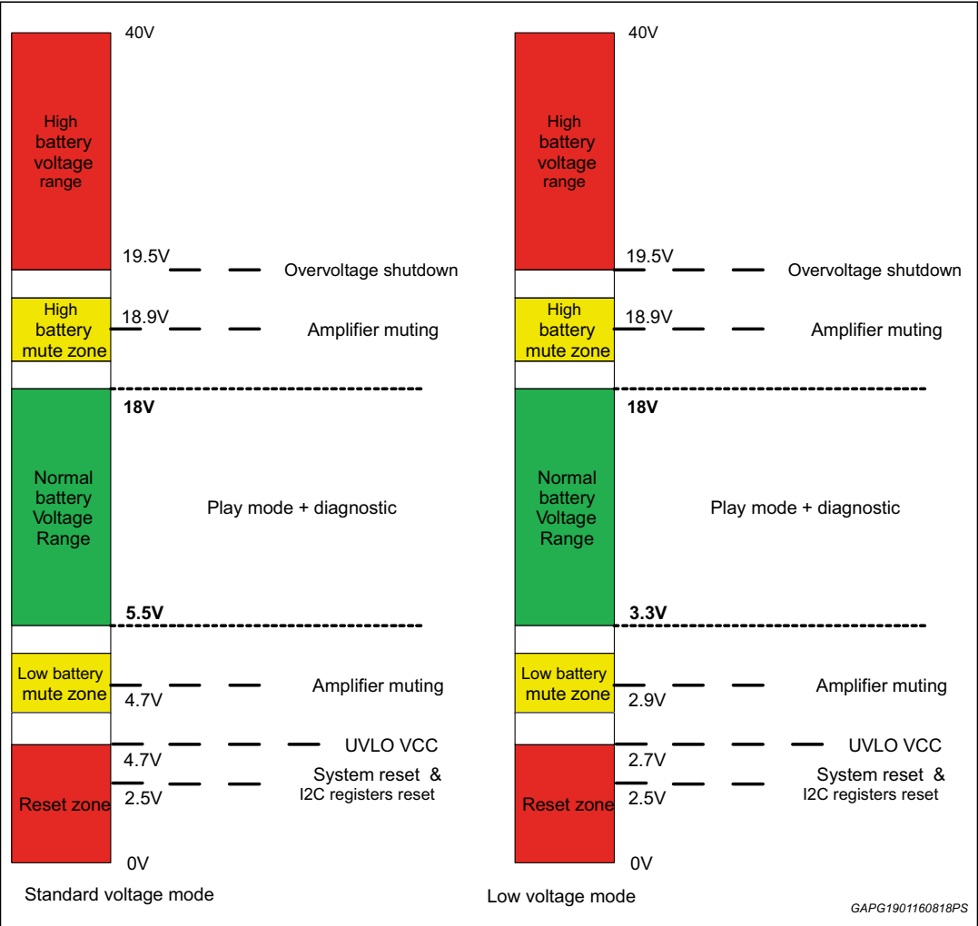
Figure 42. Operation vs. battery charge
