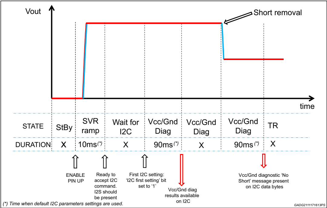
Figure 51. Short to VCC at device turn on
