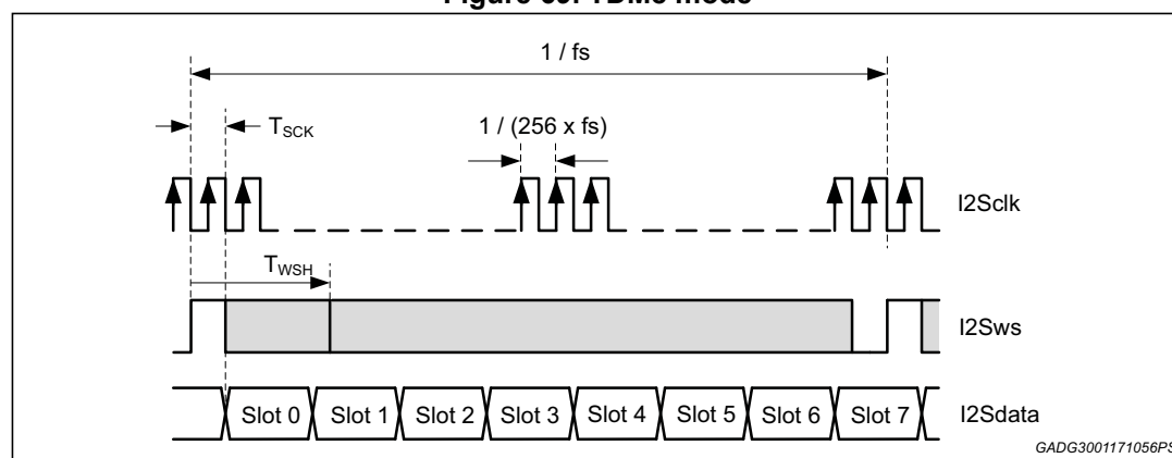
Figure 69. TDM8 mode
