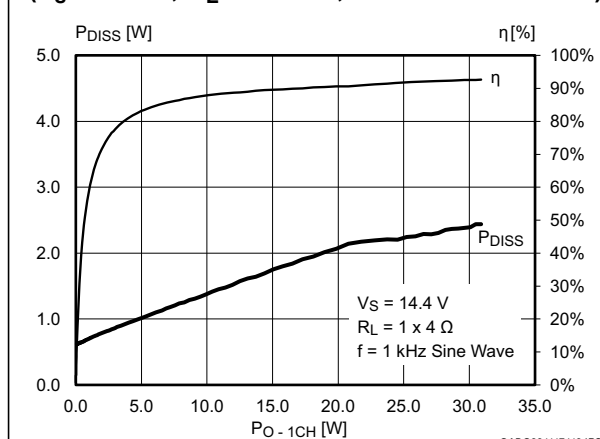
Figure 4. Efficiency and power dissipation ( V_S = 14.4 V, R_L = 1 \times 4 Ω, f = 1 kHz sine wave)
