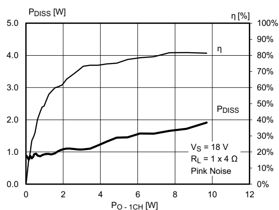
Figure 11. Efficiency and power dissipation ( V_S = 18\text{ V} , R_L = 1 \times 4\ \Omega , pink noise)
