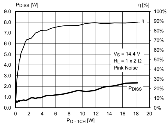
Figure 7. Efficiency and power dissipation ( V_S = 14.4\text{ V} , R_L = 1 \times 2\ \Omega , pink noise)
