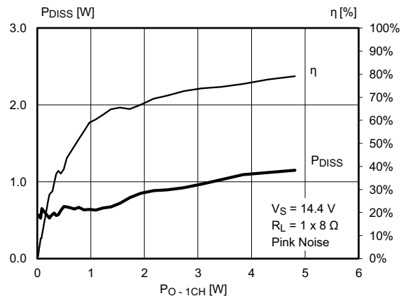
Figure 9. Efficiency and power dissipation ( V_S = 14.4\text{ V} , R_L = 1 \times 8\ \Omega , pink noise)
