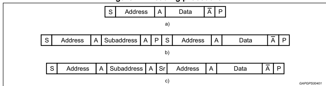
Figure 74. Reading procedure
