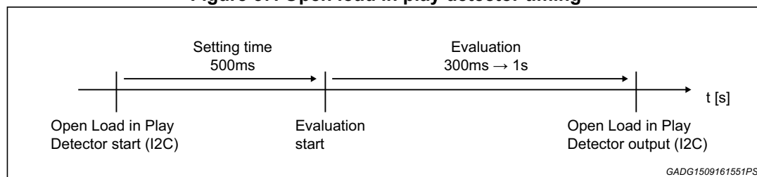
Figure 57. Open load in play detector timing
