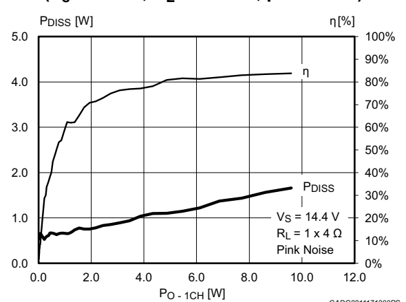
Figure 5. Efficiency and power dissipation ( V_S = 14.4 V, R_L = 1 \times 4 Ω, pink noise)
