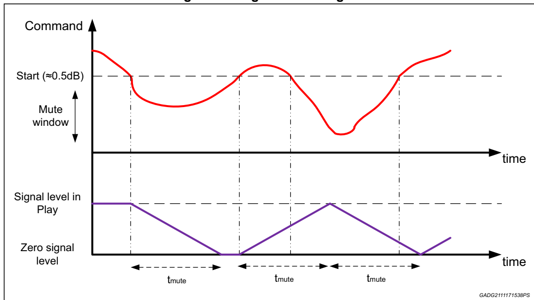
Figure 44. Digital-Mute diagram
