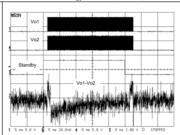
Figure 57. Startup & shutdown time V_{CC} = 5\text{ V} , G = 6\text{ dB} , C_{in} = 100\text{ nF} (5 ms/div)
