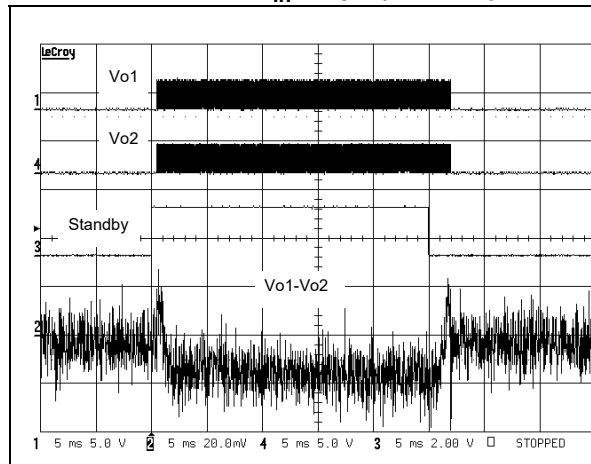
Figure 56. Startup & shutdown time V_{CC} = 3\text{ V} , G = 6\text{ dB} , C_{in} = 1\text{ }\mu\text{F} (5 ms/div)
