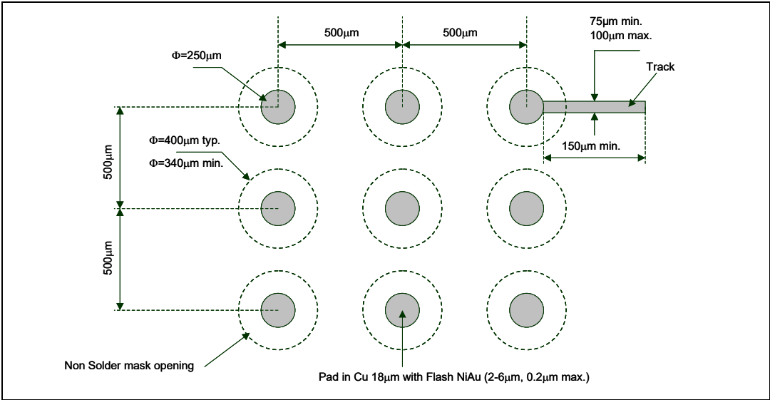
Figure 66. Footprint recommendations
