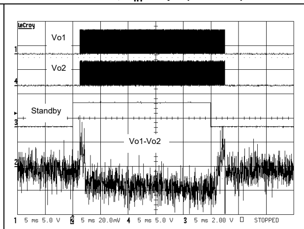
Figure 55. Startup & shutdown time V_{CC} = 5\text{ V} , G = 6\text{ dB} , C_{in} = 1\text{ }\mu\text{F} (5 ms/div)
