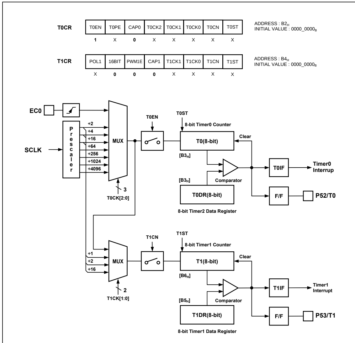
Figure 11-6 8 Bit Timer/Event Counter2, 3 Block Diagram
