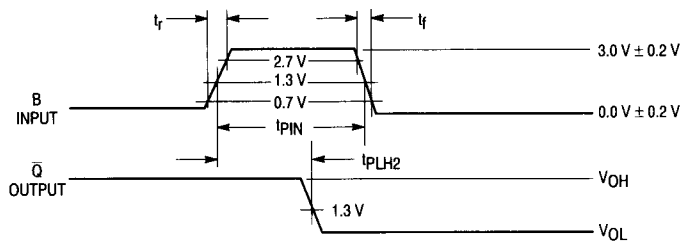
t_{PLH2} Waveforms
