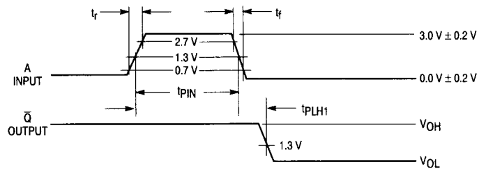
t_{PLH1} Waveforms
