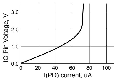
Figure 24: Typical internal pull-down and pull-up currents
