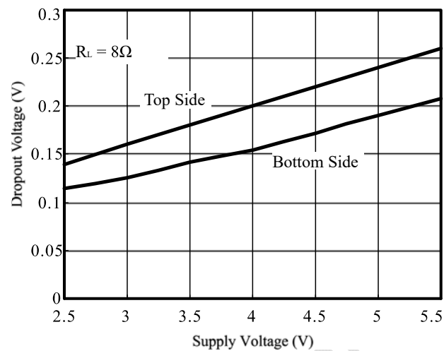
Figure 16 Dropout Voltage vs. Supply Voltage
