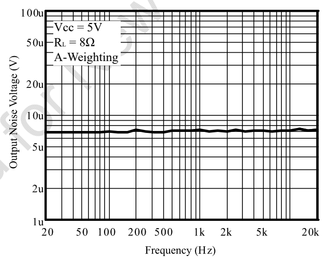
Figure 11 Noise Floor
