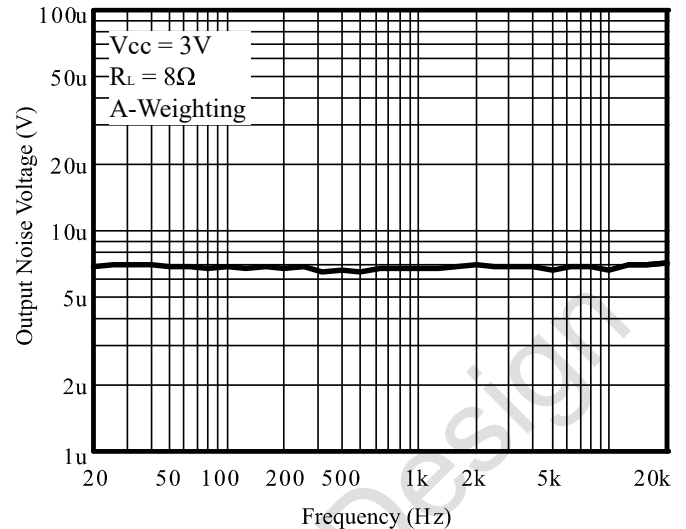
Figure 15 Noise Floor
