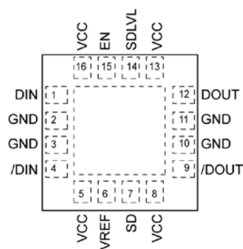
16-Pin QFN
