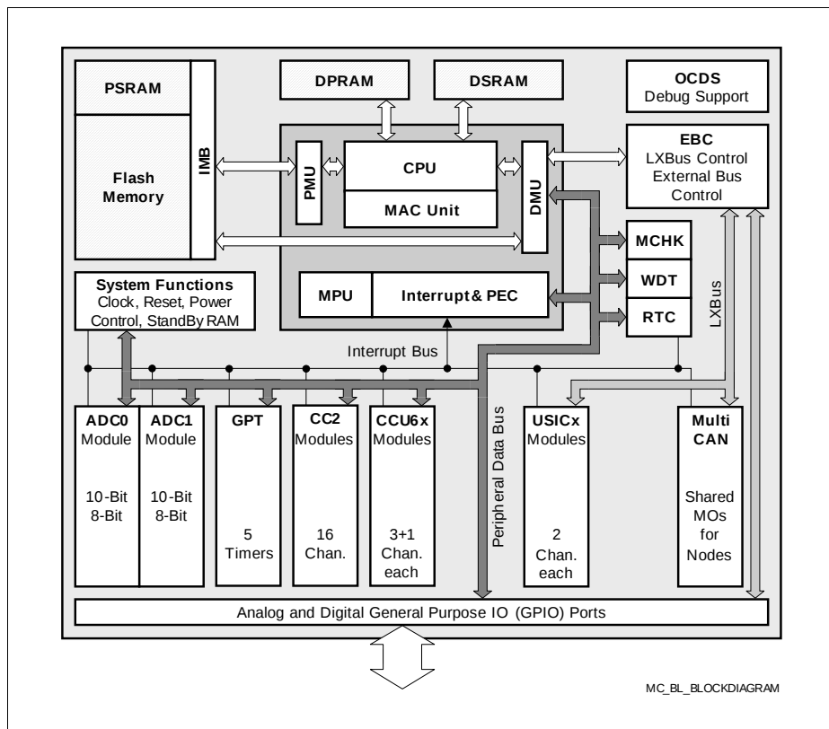
Figure 6 Block Diagram
