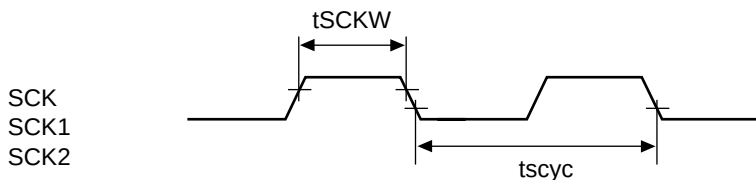
Figure 23.52 Input Clock Input/Output Timing
