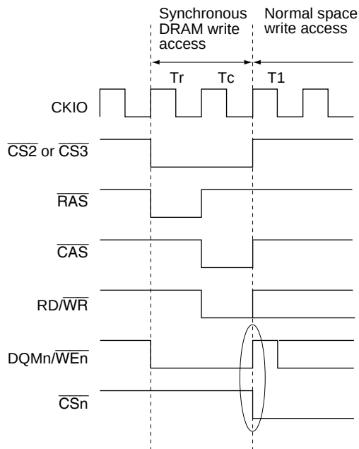
Figure 7.58 Normal Space Access after Synchronous DRAM Write (Single Write Mode)
