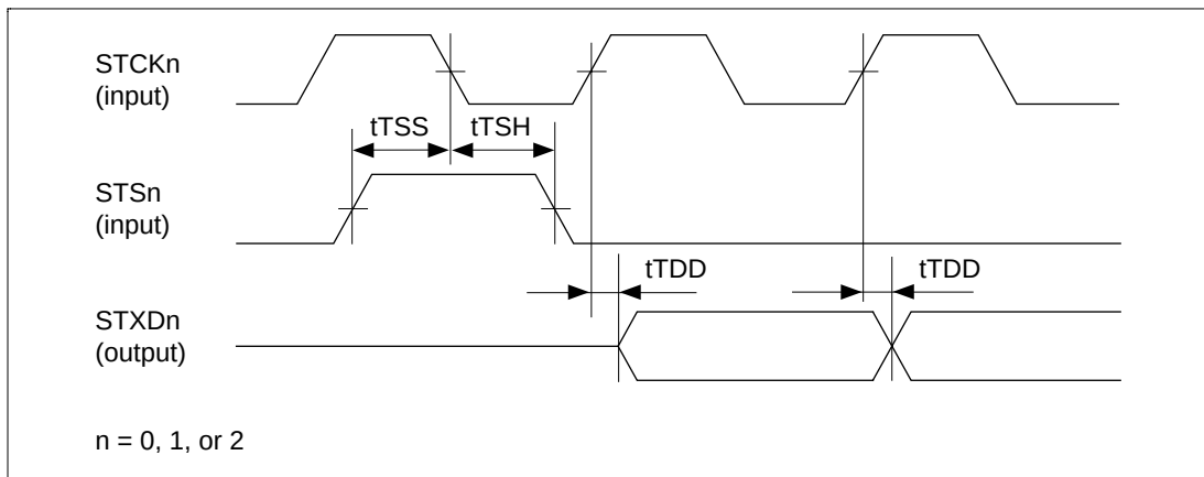
Figure 23.62 SIO Transmit Timing (TMn = 0 Mode)
