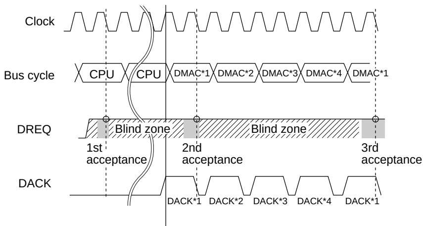
Figure 9.42 DREQ Pin Input Detection Timing in Burst Mode with Level Detection (16-Byte Transfer Setting)
