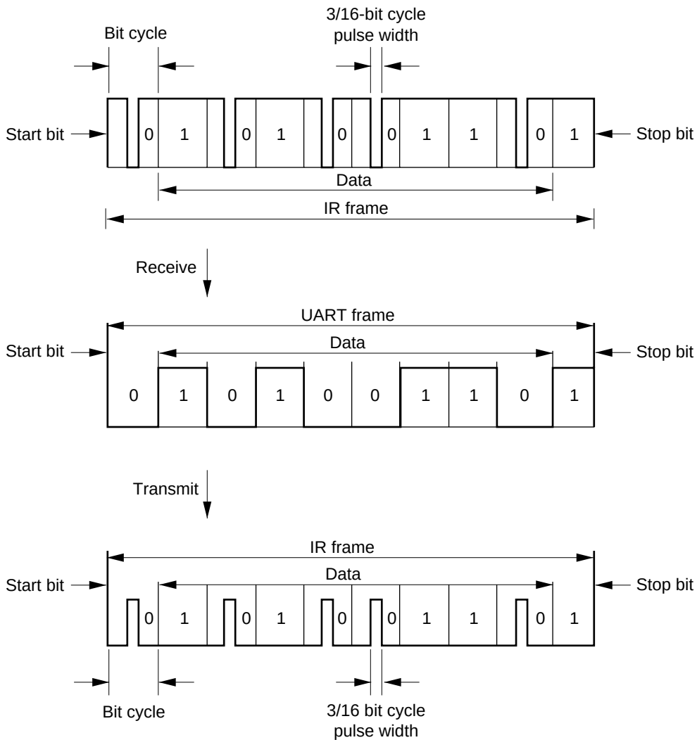
Figure 16.2 Transmit/Receive Operation
