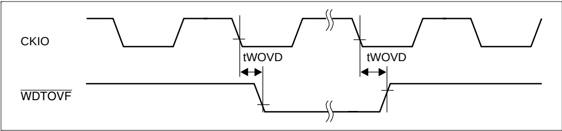
Figure 23.59 Watchdog Timer Output Timing (tEcyc:tPcyc ≠ 1:1)
