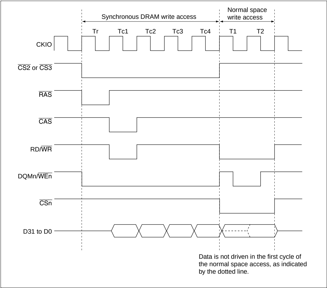
Figure 9.52 Normal Space Access (No Wait)
