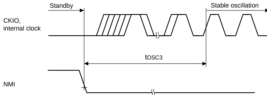
Figure 23.6 Oscillation Stabilization Time after Standby Recovery (Recovery by NMI)
