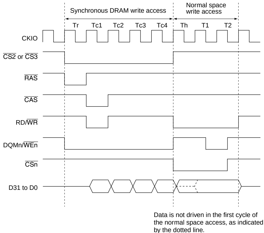
Figure 7.56 Normal Space Access (One Setup Wait Cycle)
