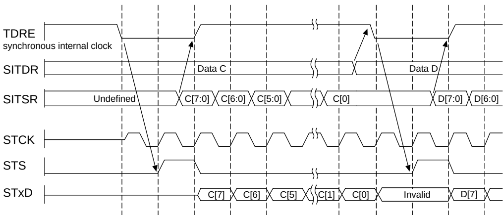
Figure 17.5 Transmission: Continuous Transfer Mode (TM = 0 Mode)
