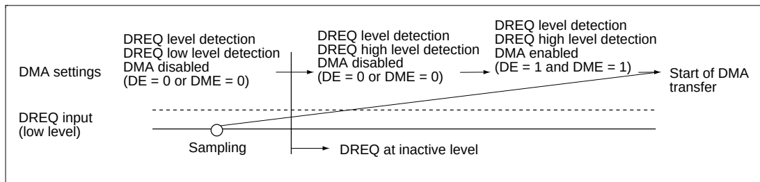
Figure 9.43 Initiation of DMA Transfer (1)
