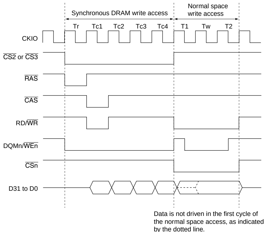
Figure 9.53 Normal Space Access (One Wait)
