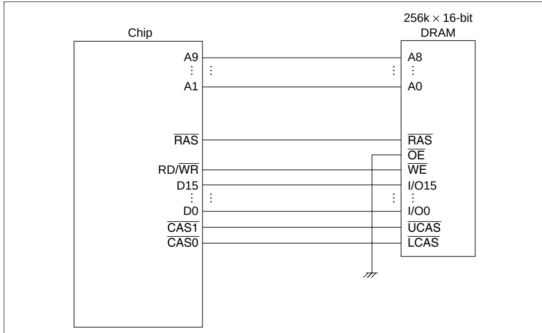
Figure 7.35 Example of DRAM Connection (16-Bit Data Width)
