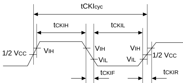
Figure 23.2 CKIO Clock Input Timing
