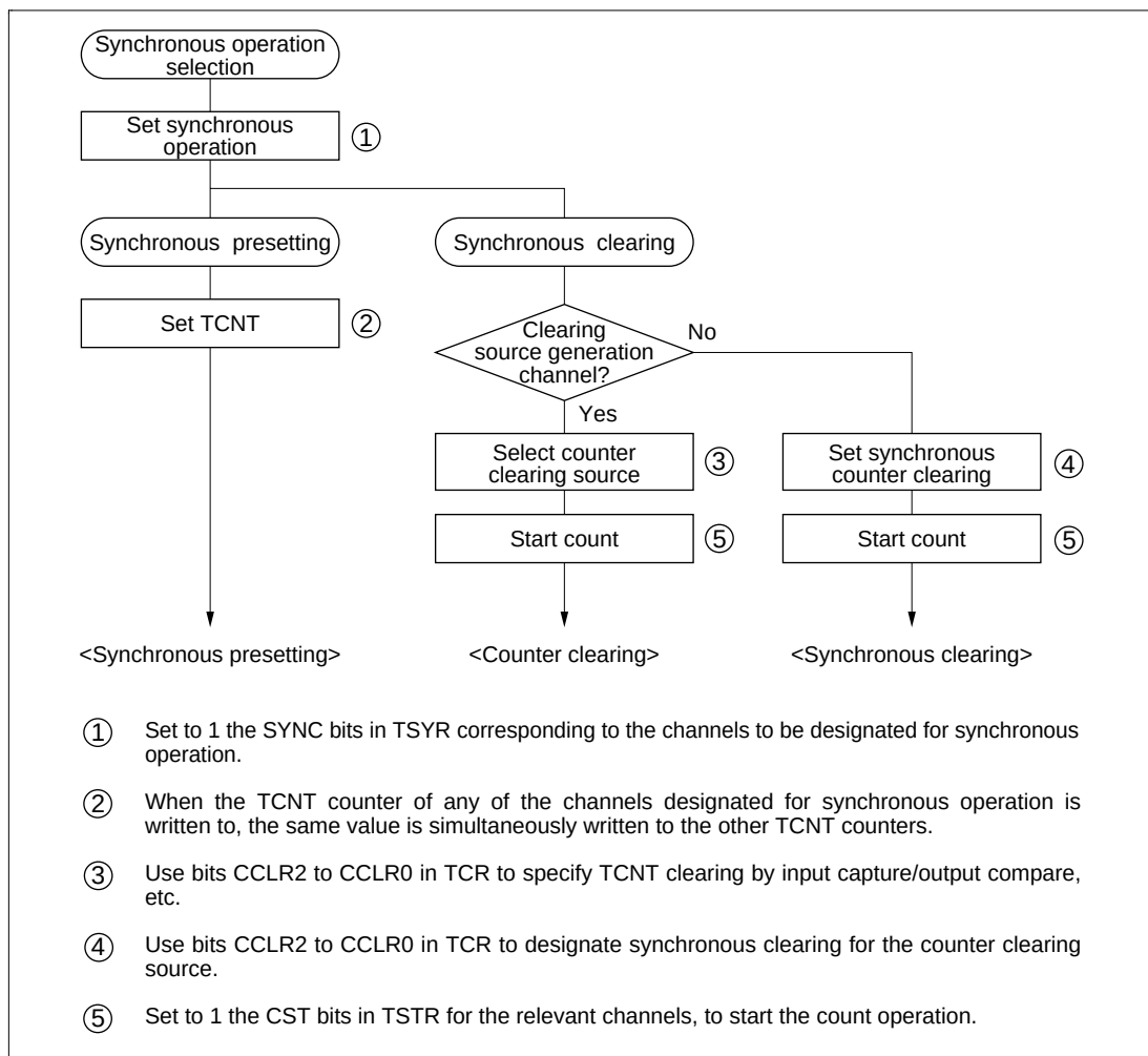
Figure 18.14 Example of Synchronous Operation Setting Procedure
