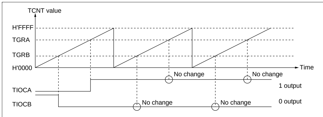
Figure 18.10 Example of 0 Output/1 Output Operation
