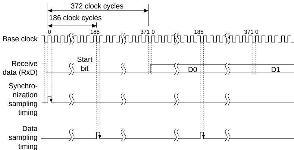
Figure 14.11 Receive Data Sampling Timing in Smart Card Mode
