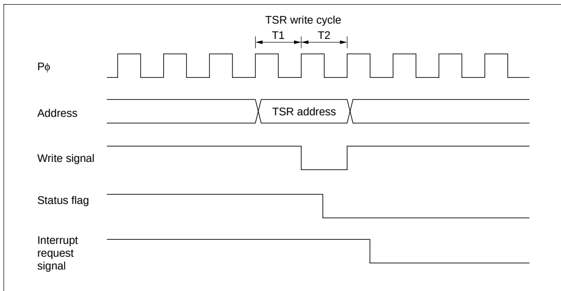
Figure 18.42 Timing for Status Flag Clearing by CPU
