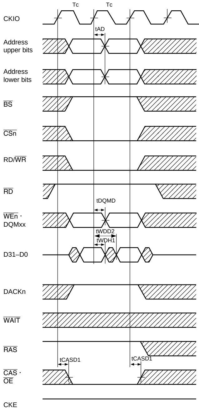
Figure 23.27 Synchronous DRAM Continuous Write Cycle (Bank Active, Same Row Access, I\phi:E\phi = 1:1 )
