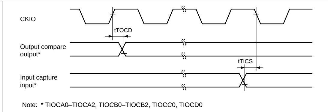
Figure 23.55 TPU Input/Output Timing ( t_{Ecyc}:t_{Pcyc} = 1:1 )
