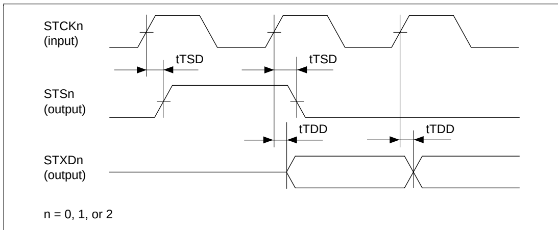
Figure 23.63 SIO Transmit Timing (TMn = 1 Mode)
