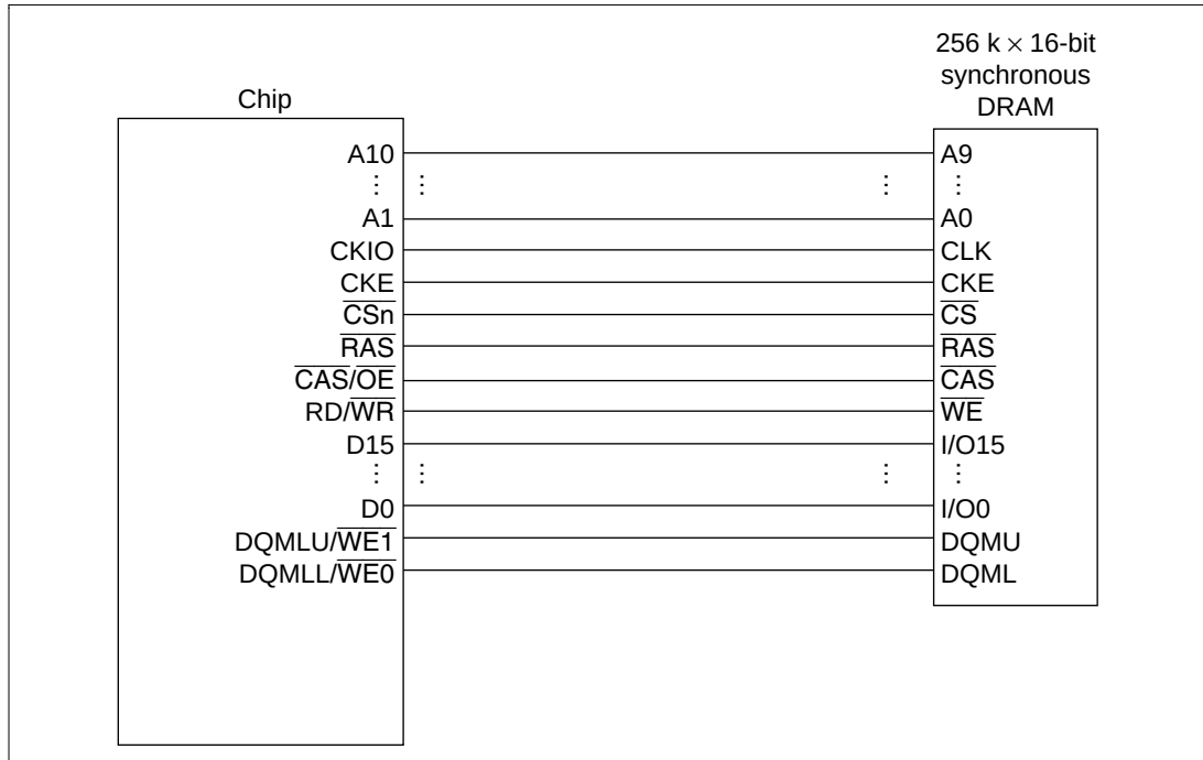
Figure 7.19 Synchronous DRAM 16-bit Device Connection
