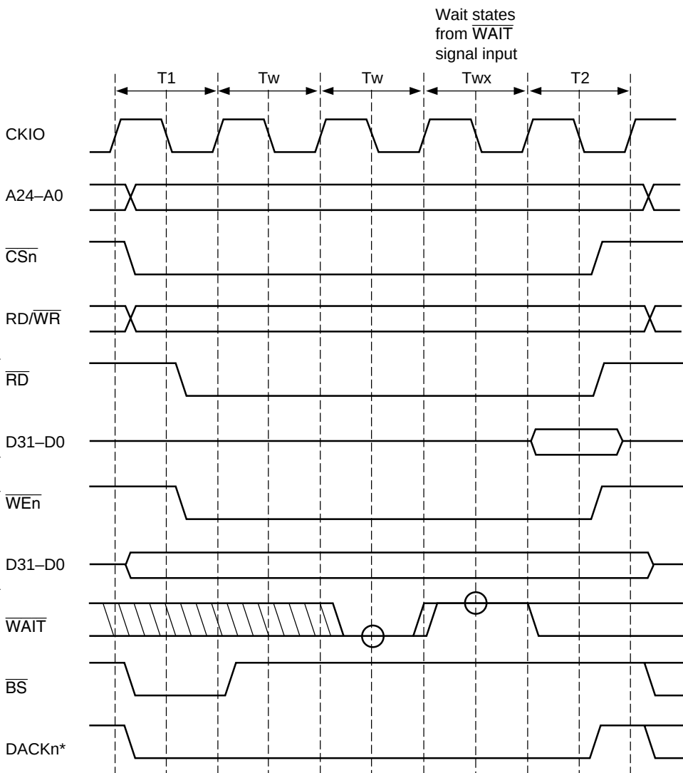
Figure 7.15 Wait State Timing of Ordinary Space Access (Wait States from \overline{\text{WAIT}} Signal)
