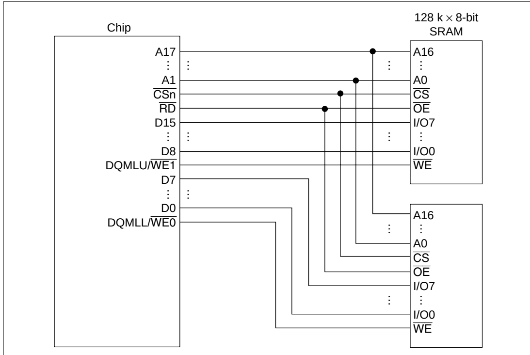
Figure 7.12 Example of 16-Bit Data Width SRAM Connection
