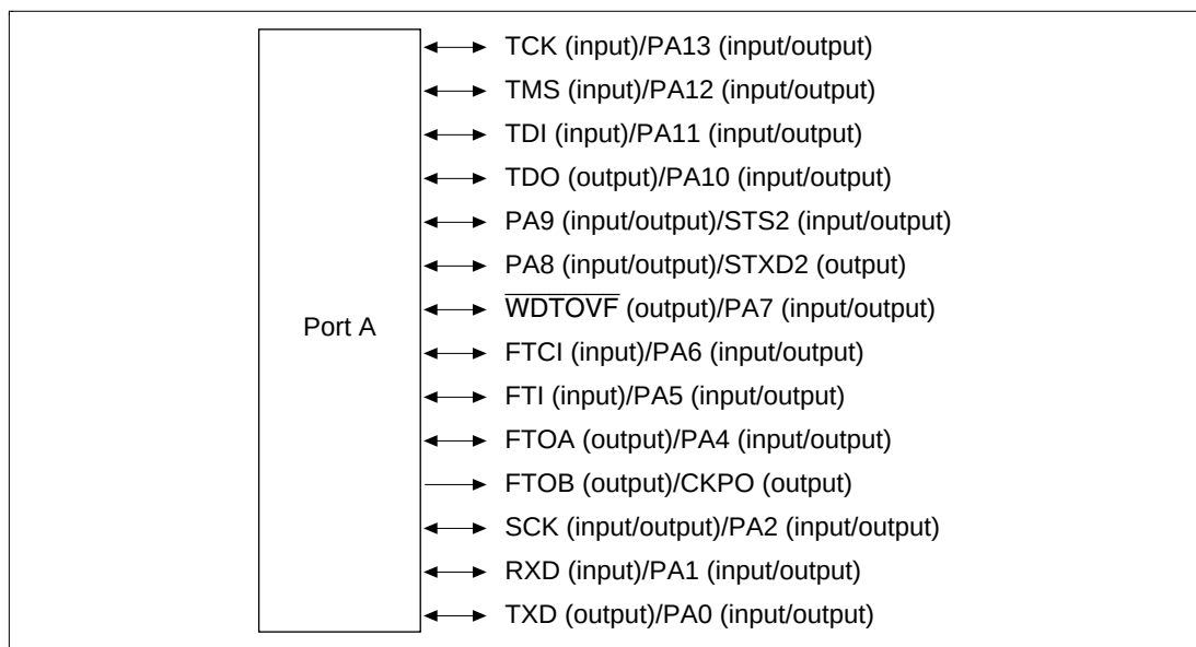
Figure 21.1 Port A
