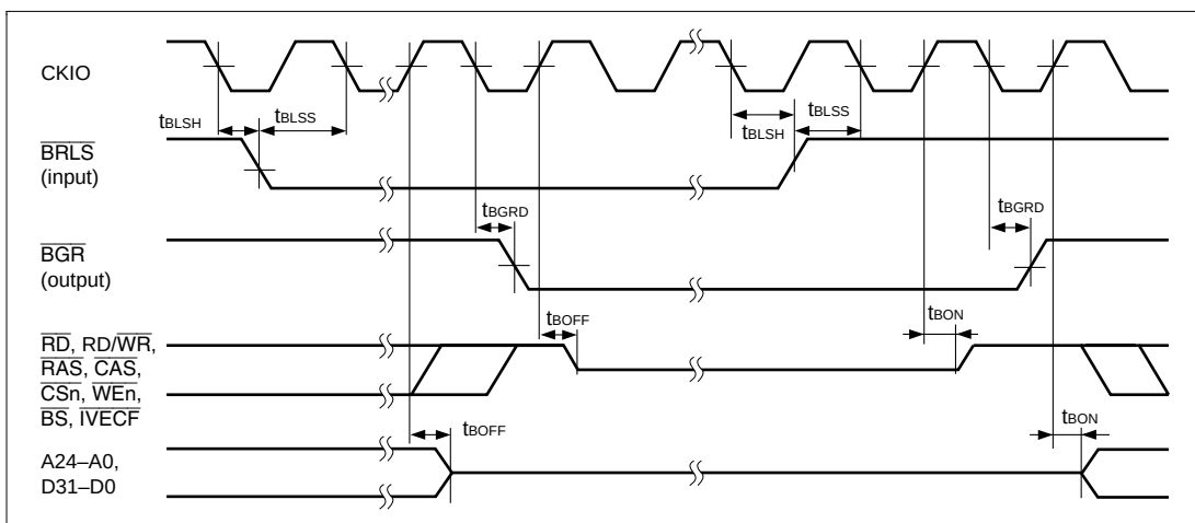
Figure 23.10 Bus Release Timing
