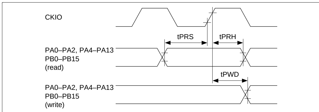
Figure 23.67 I/O Port Input/Output Timing (tEcy:c:tPcyc = 1:1)
