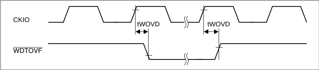
Figure 23.58 Watchdog Timer Output Timing (tEcyc:tPcyc = 1:1)
