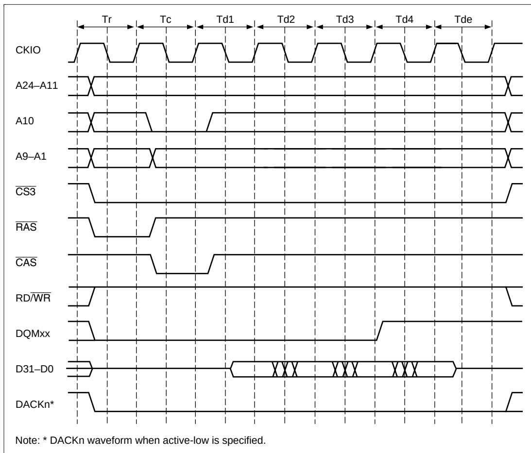
Figure 7.25 Burst Read Timing (No Precharge)
