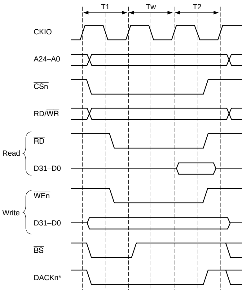
Figure 7.14 Wait Timing of Ordinary Space Access (Software Wait Only)
