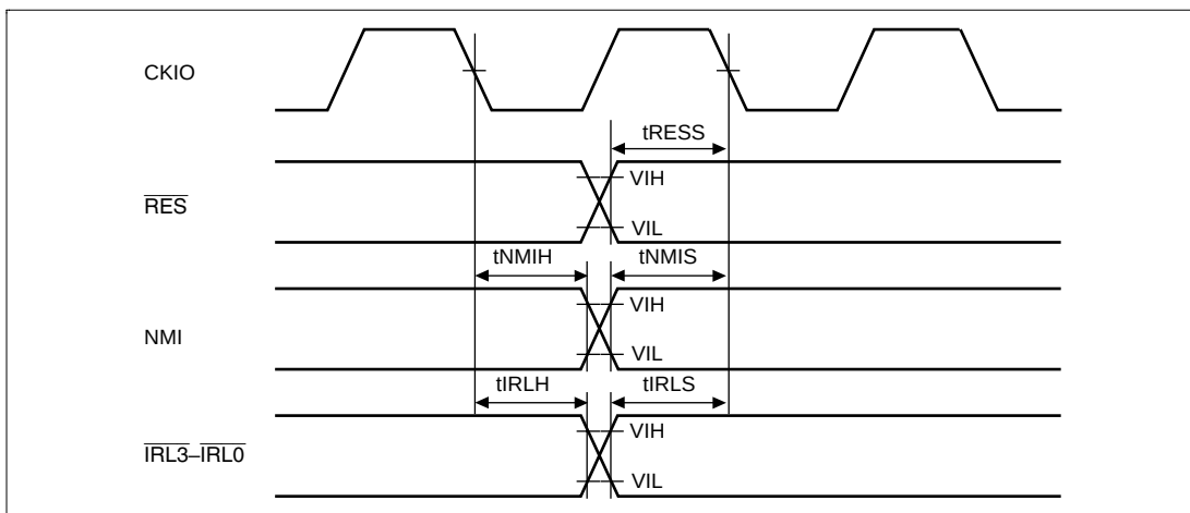
Figure 23.9 Interrupt Signal Input Timing
