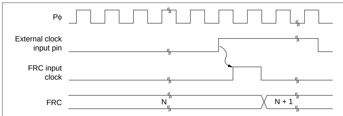
Figure 11.5 Count Timing (External Clock Operation)
