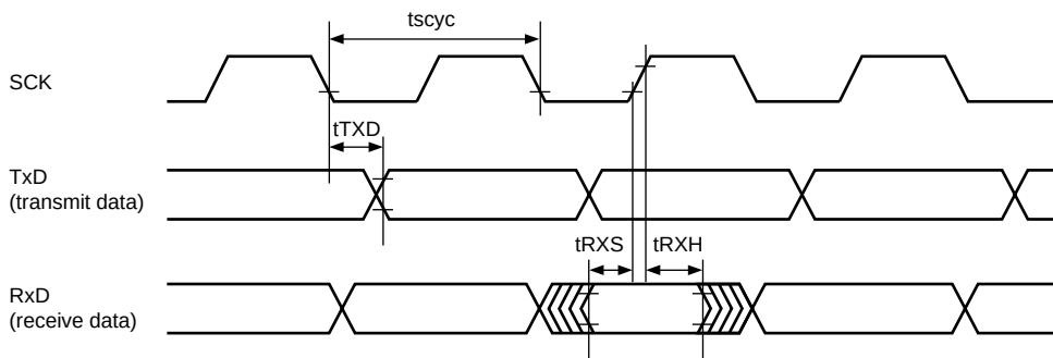
Figure 23.53 SCI Input/Output Timing (Synchronous Mode)
