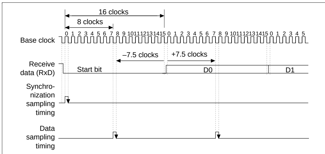
Figure 15.9 Receive Data Sampling Timing in Asynchronous Mode
