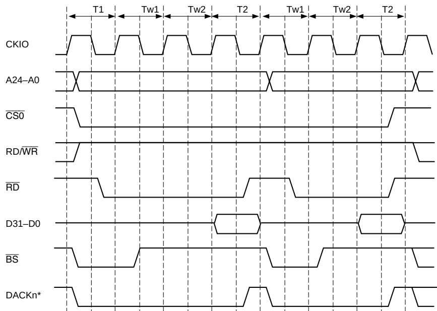
Figure 7.50 Burst ROM Nibble Access (2 Wait States)
