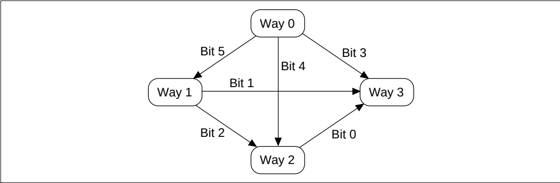
Figure 8.7 LRU Information and Access Sequence
