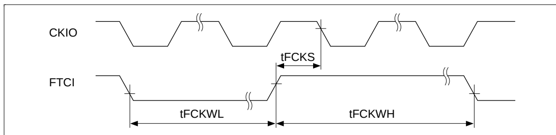
Figure 23.51 FRT Clock Input Timing ( t_{Ecyc}:t_{Pcyc} \neq 1:1 )
