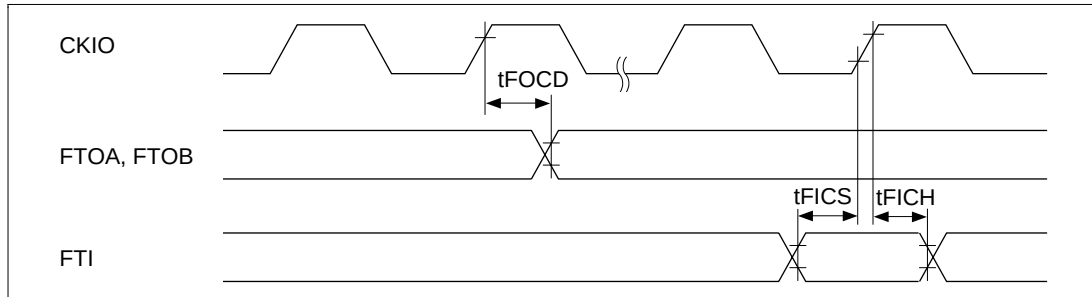
Figure 23.48 FRT Input/Output Timing ( t_{Ecyc}:t_{Pcyc} = 1:1 )
