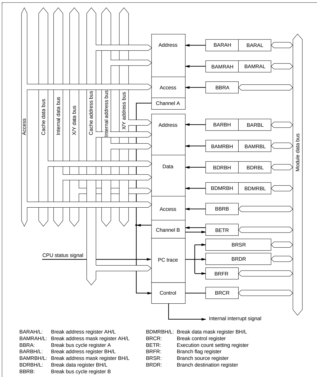
Figure 6.1 User Break Controller Block Diagram
