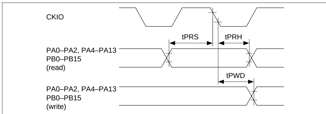
Figure 23.68 I/O Port Input/Output Timing (tEcy:c:tPcyc ≠ 1:1)
