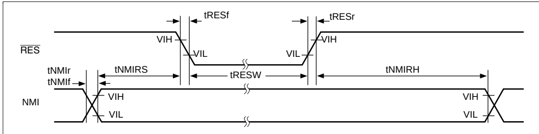
Figure 23.8 Reset Input Timing
