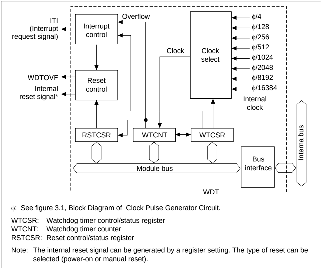
Figure 12.1 WDT Block Diagram
