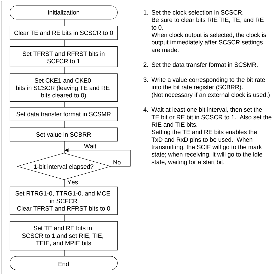
Figure 15.2 Sample Flowchart for SCIF Initialization
