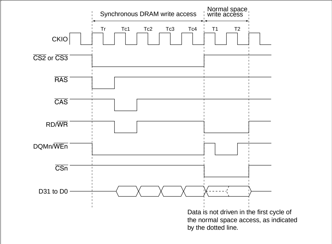
Figure 7.54 Normal Space Access (No Wait)
