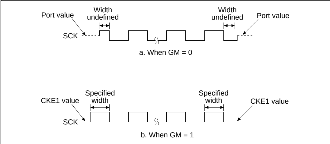
Figure 14.7 Difference in Clock Output According to GM Bit Setting
