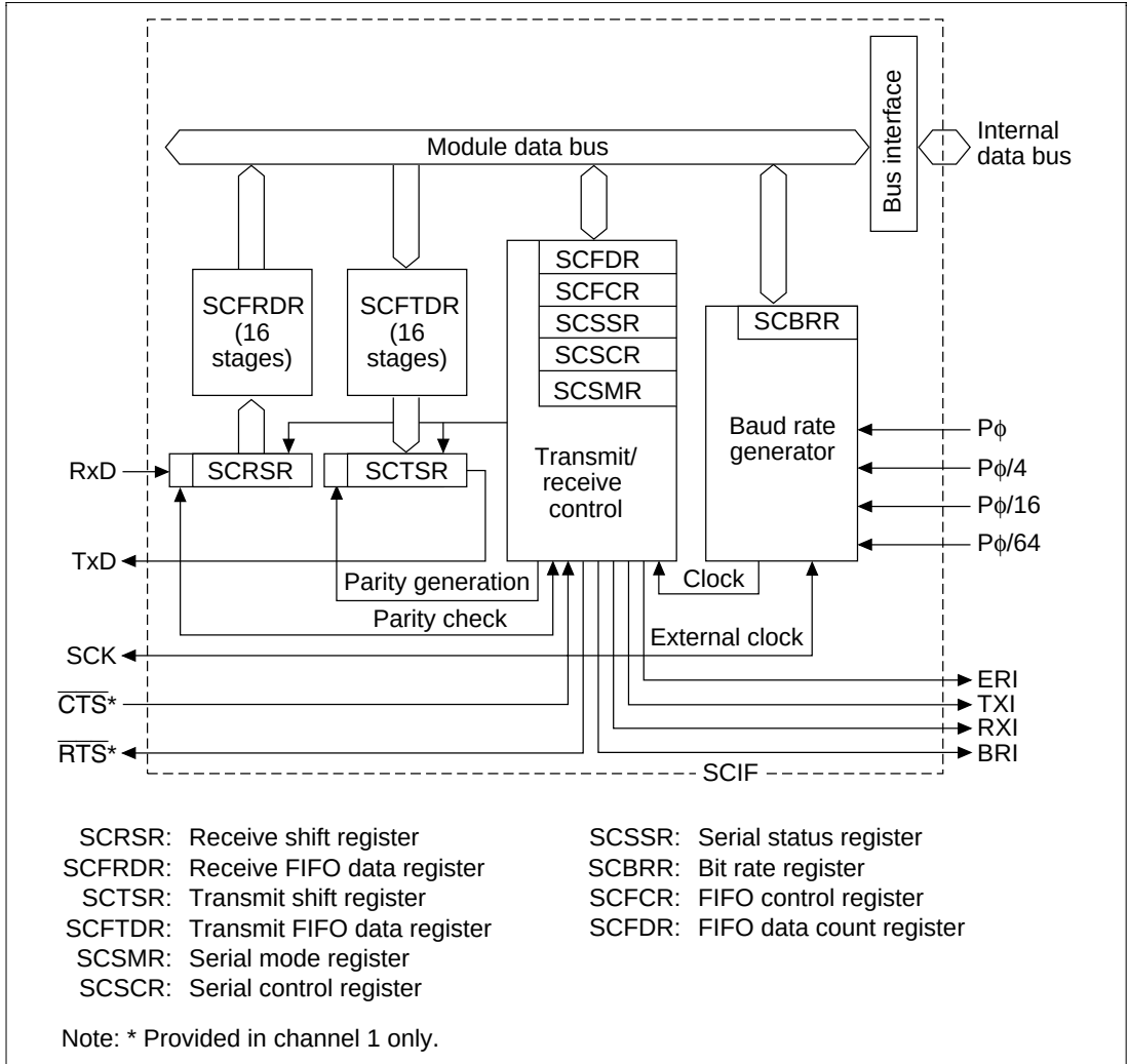
Figure 15.1 SCIF Block Diagram
