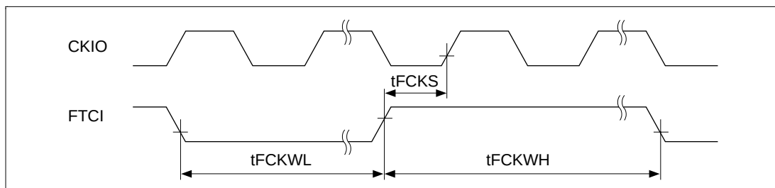
Figure 23.50 FRT Clock Input Timing ( t_{Ecyc}:t_{Pcyc} = 1:1 )
