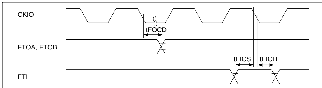
Figure 23.49 FRT Input/Output Timing ( t_{Ecyc}:t_{Pcyc} \neq 1:1 )
