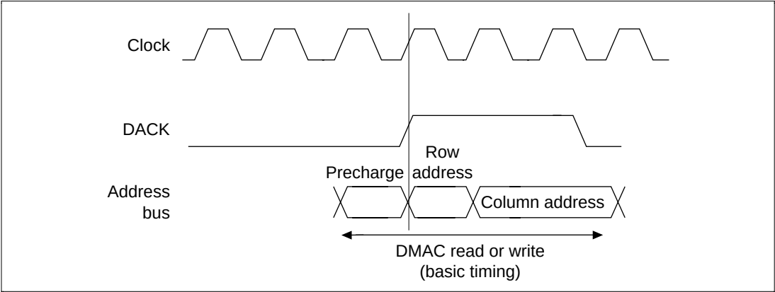
Figure 9.29 DACK Output in Normal DRAM Accesses (AM = 0 or 1)
