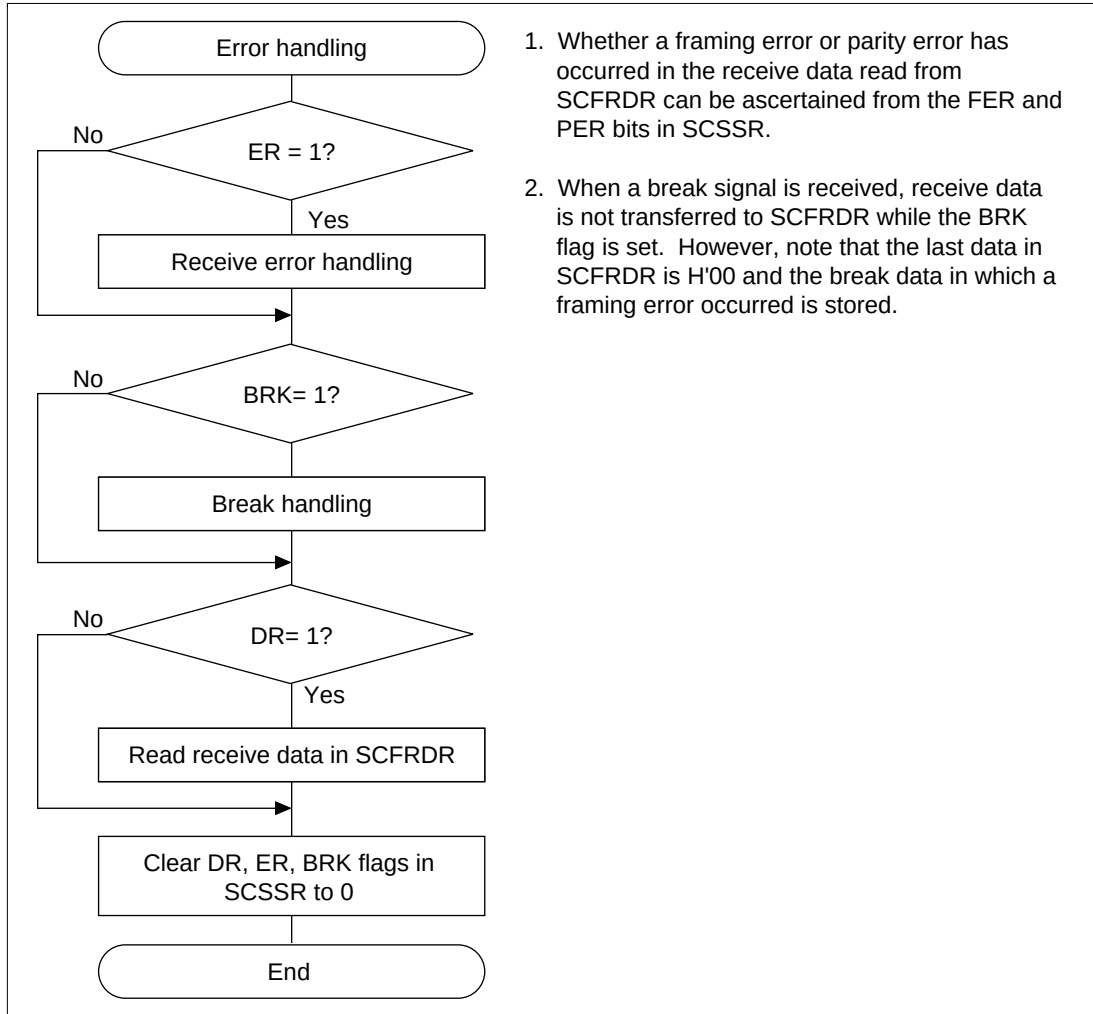
Figure 15.6 Sample Flowchart for Serial Reception (cont)
