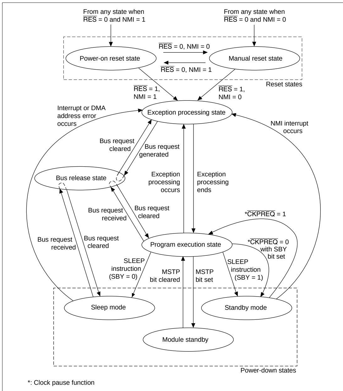
Figure 1.4 Transitions between Processing States
