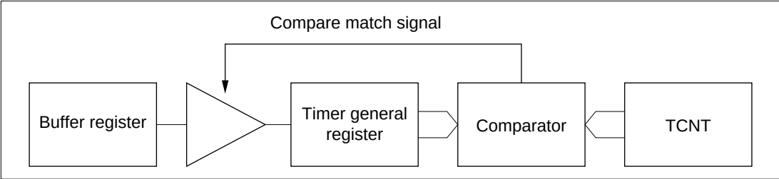
Figure 18.16 Compare Match Buffer Operation
