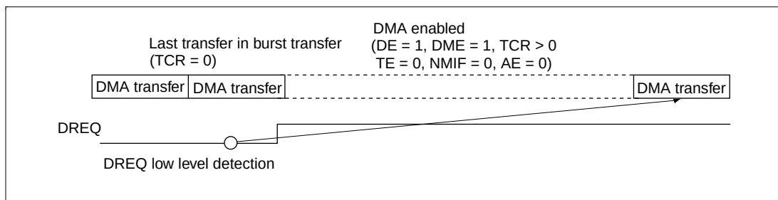
Figure 9.44 Initiation of DMA Transfer (2)
