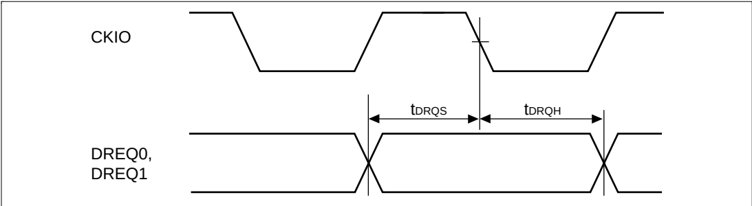
Figure 23.47 DREQ0, DREQ1 Input Timing
