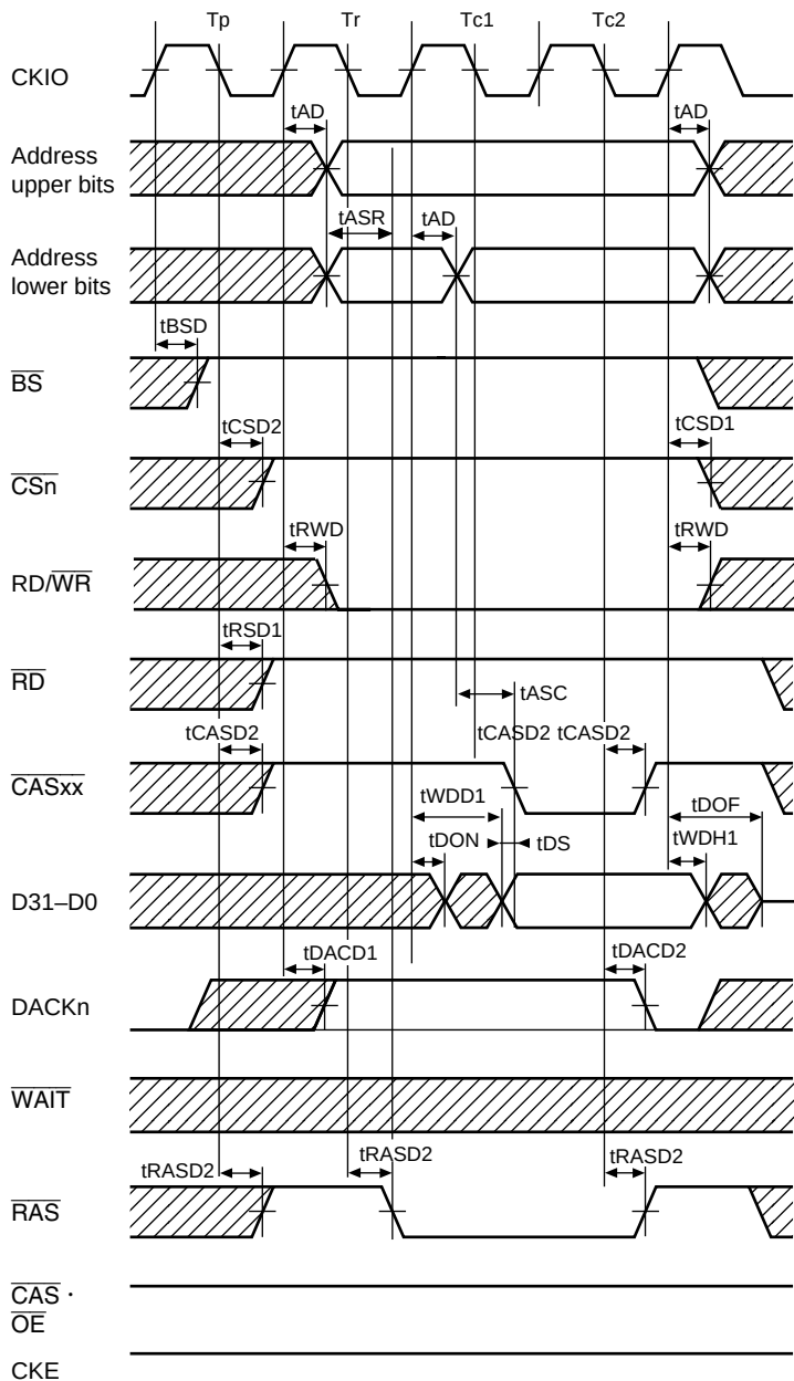
Figure 23.34 DRAM Write Cycle (TRP = 1 Cycle, RCD = 1 Cycle, No Wait)
