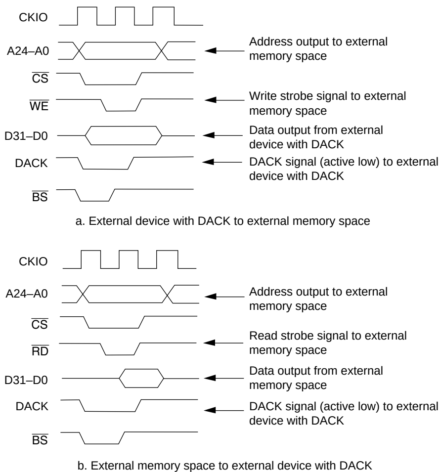
Figure 9.7 DMA Transfer Timing in Single Address Mode
