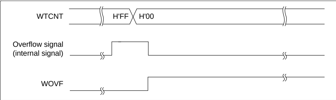
Figure 12.7 Timing of WOVF Setting
