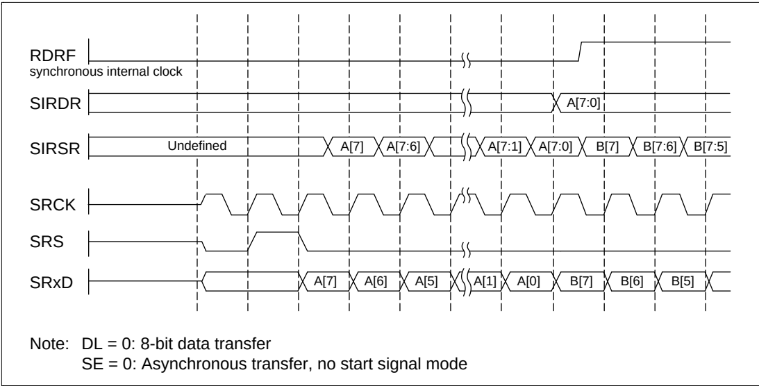
Figure 17.3 Reception: Continuous Transfer Mode
