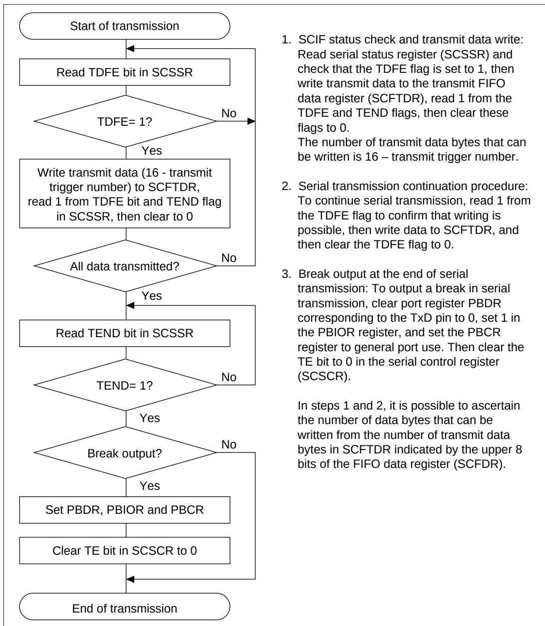
Figure 15.3 Sample Flowchart for Serial Transmission
