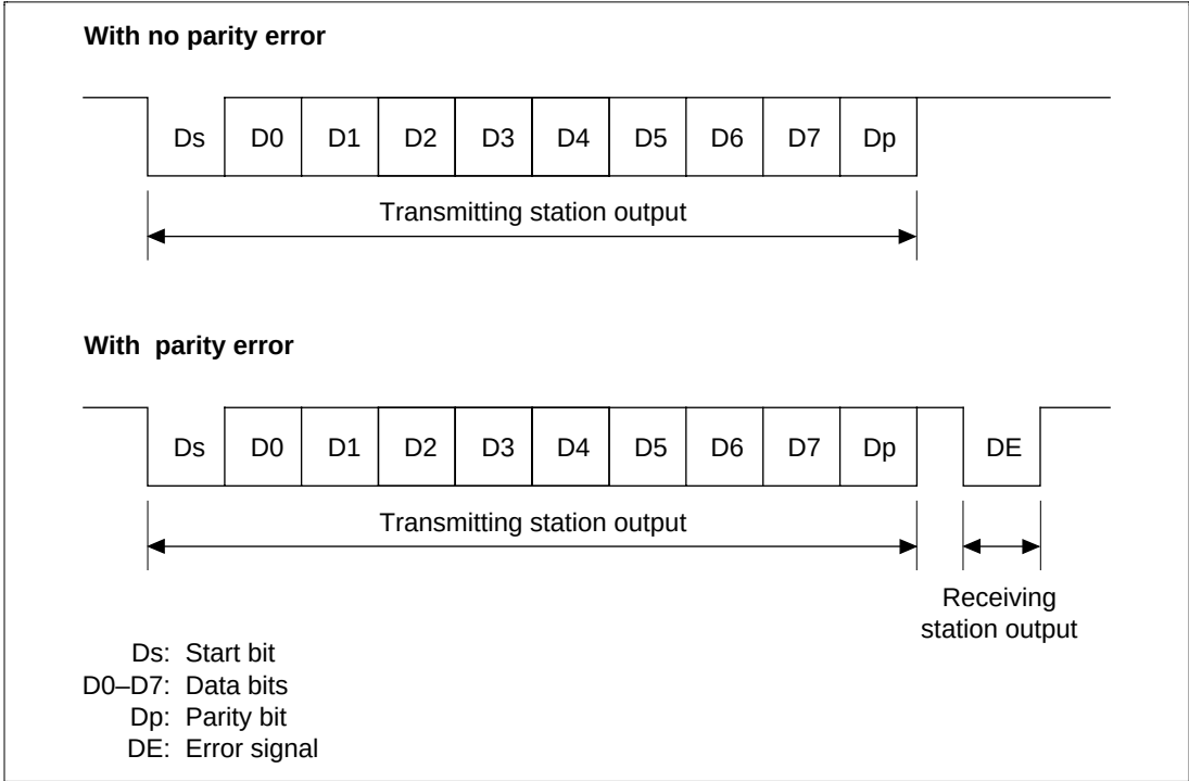
Figure 14.5 Data Format for Smart Card Interface
