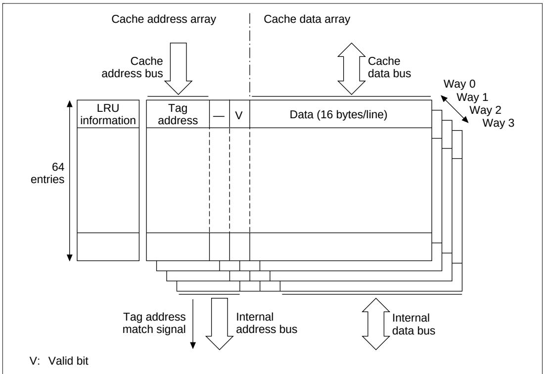
Figure 8.1 Cache Configuration
