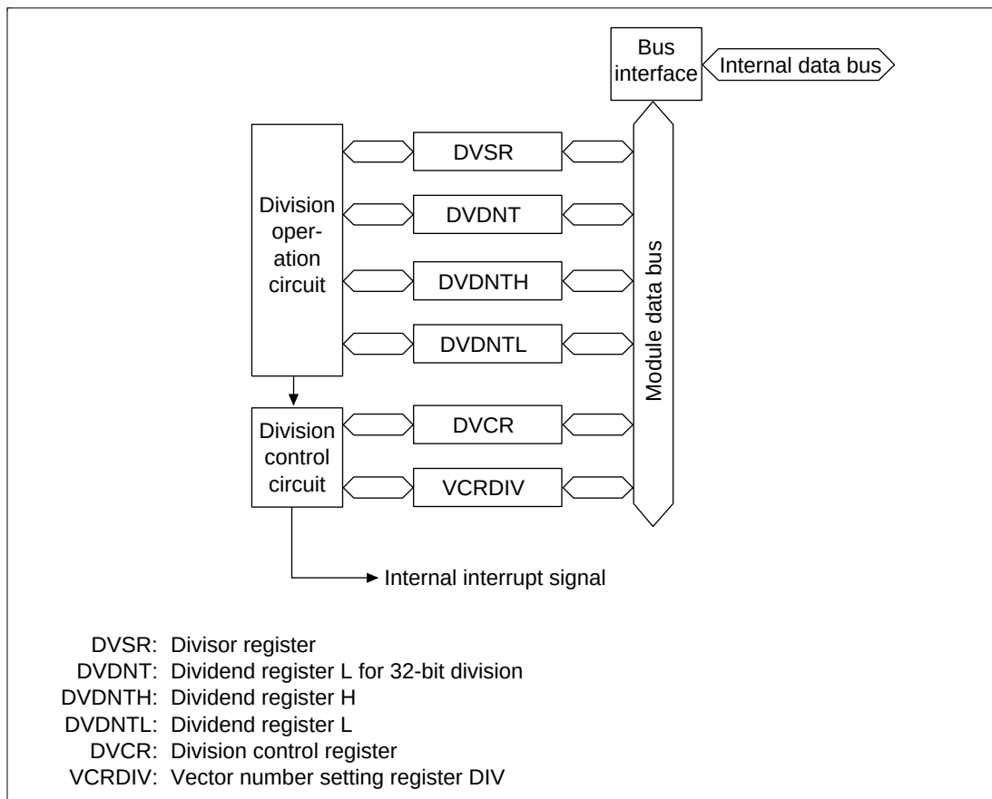
Figure 10.1 DIVU Block Diagram
