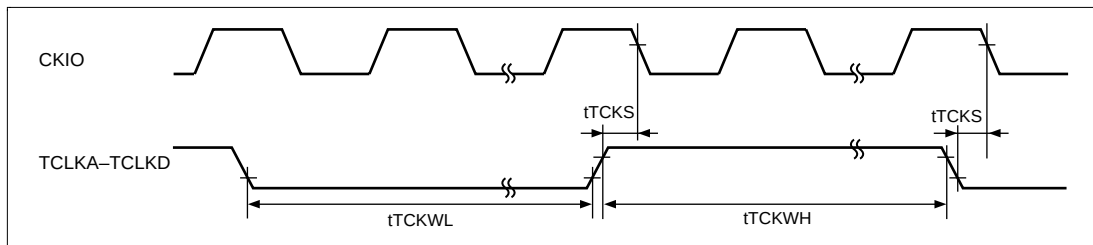
Figure 23.57 TPU Clock Input Timing
