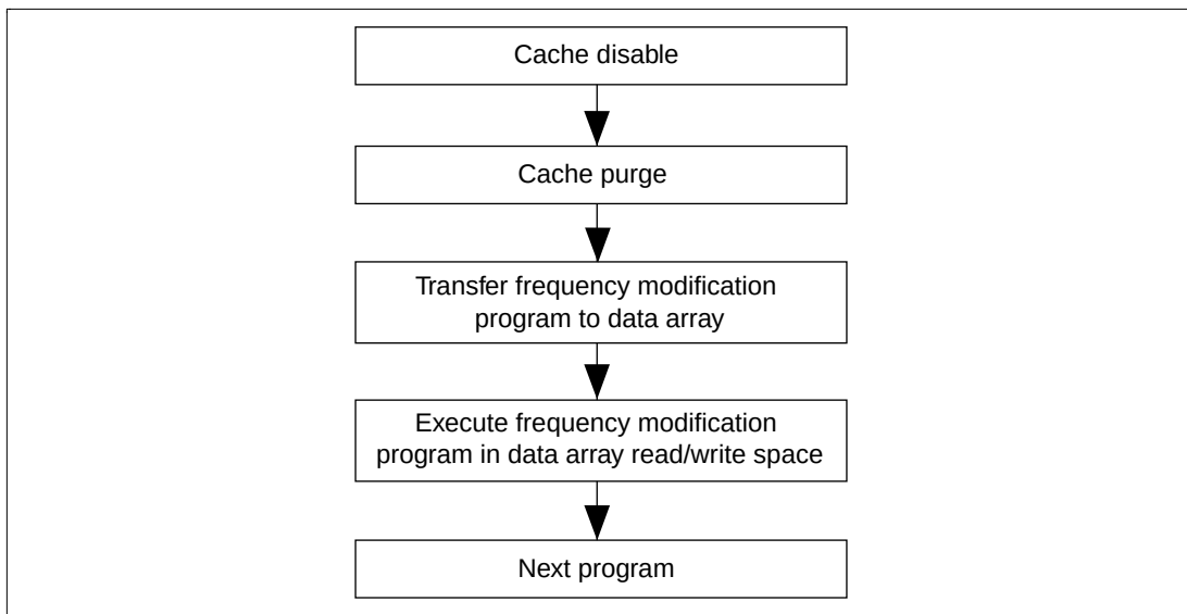
Figure 3.5 Frequency Modification Flowchart
