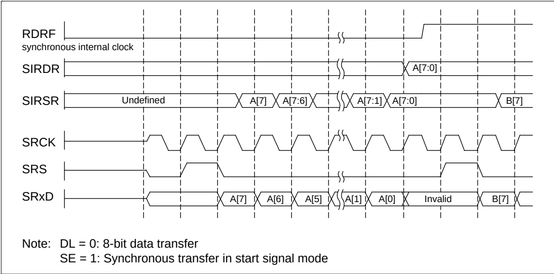
Figure 17.2 Reception: Interval Transfer Mode
