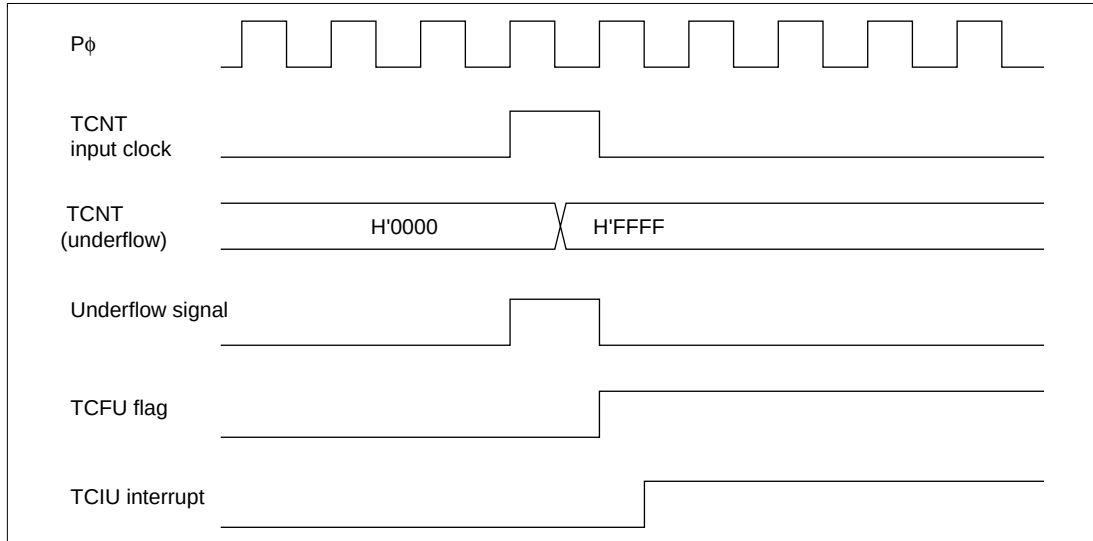
Figure 18.41 TCIU Interrupt Setting Timing
