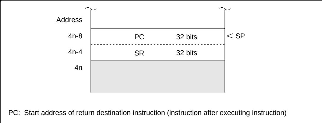
Figure 5.9 Stack State after Interrupt Exception Handling
