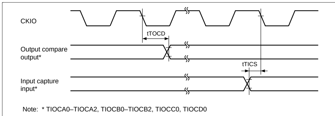
Figure 23.56 TPU Input/Output Timing ( t_{Ecyc}:t_{Pcyc} \neq 1:1 )
