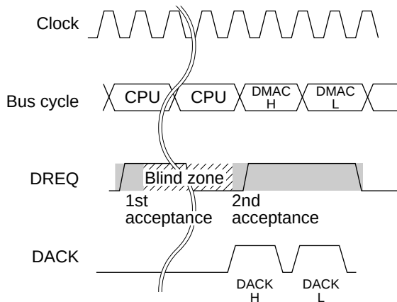
Figure 9.34 When a 16-Bit External Device is Connected (Edge Detection)
