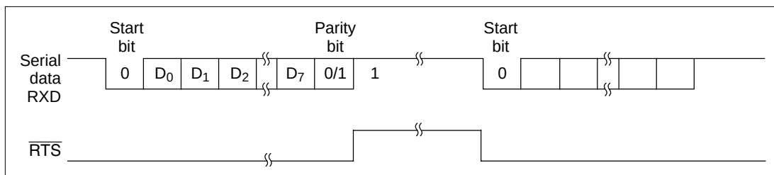
Figure 15.8 Example of Operation Using Modem Control ( \overline{\text{RTS}} )
