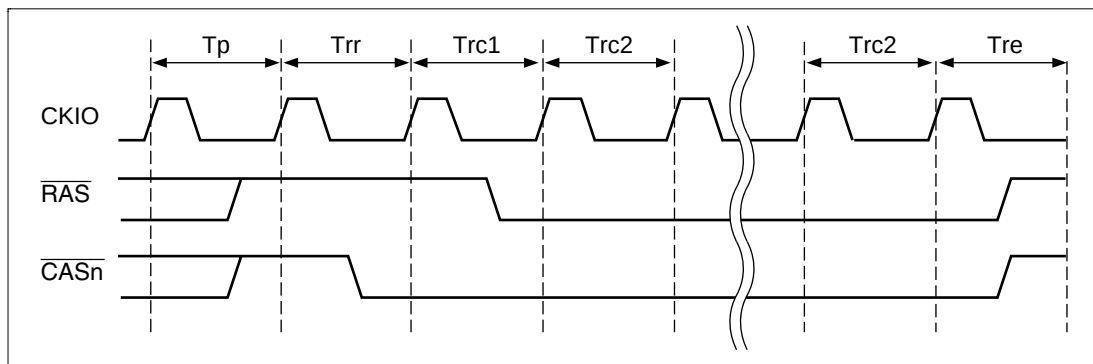
Figure 7.48 DRAM Self-Refresh Cycle Timing
