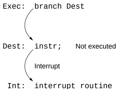
Figure 6.2 When Interrupt Occurs before Branch Instruction is Executed
