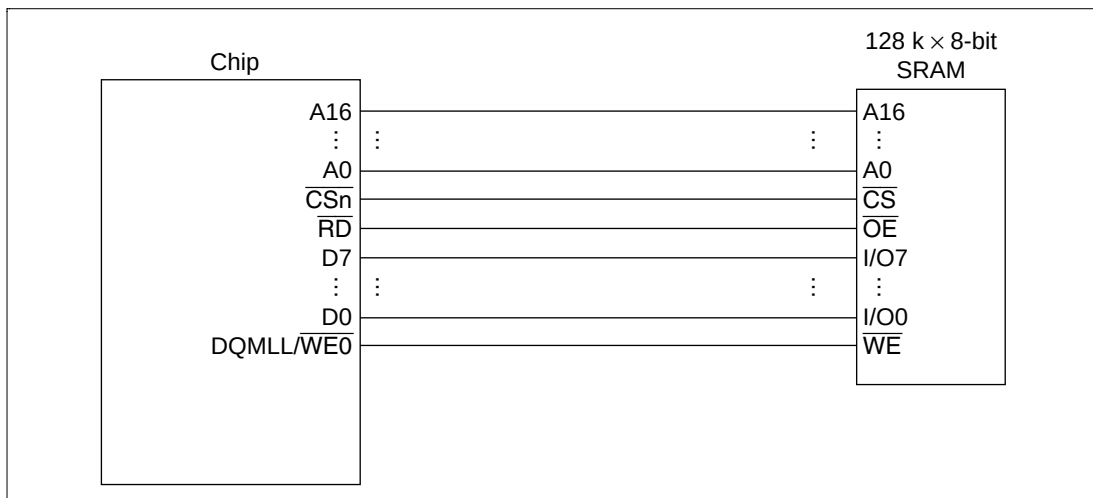
Figure 7.13 Example of 8-Bit Data Width SRAM Connection
