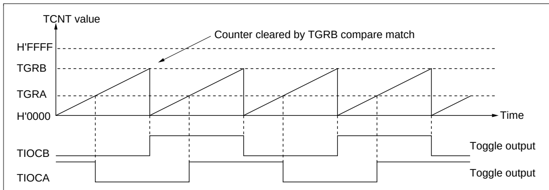
Figure 18.11 Example of Toggle Output Operation
