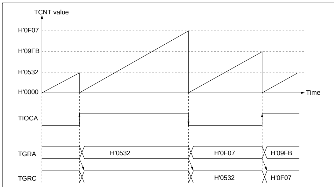
Figure 18.20 Example of Buffer Operation (2)
