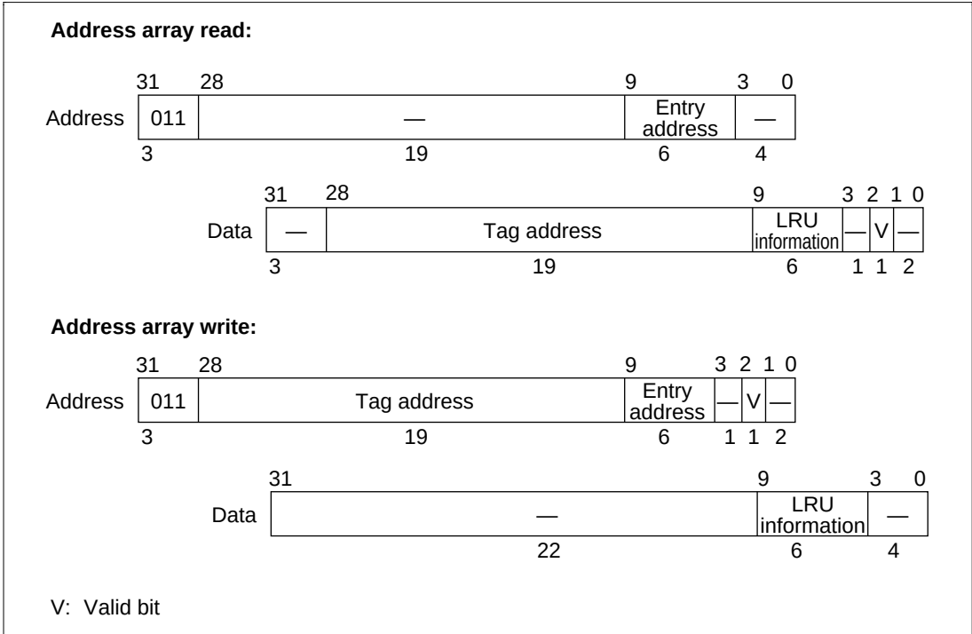
Figure 8.10 Address Array Access
