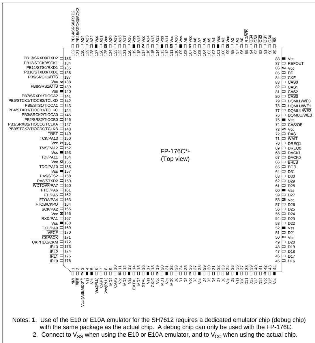
Figure 1.2 Pin Arrangement (FP-176C)
