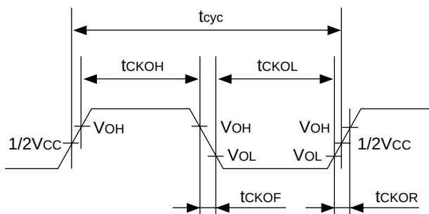
Figure 23.3 CKIO Clock Output Timing
