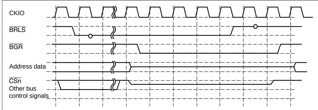
Figure 7.53 Bus Arbitration
