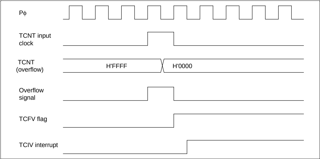
Figure 18.40 TCIV Interrupt Setting Timing
