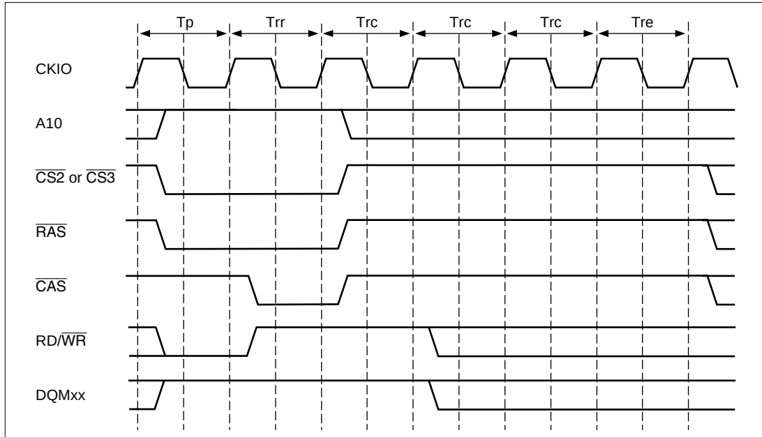
Figure 7.31 Auto-Refresh Timing
