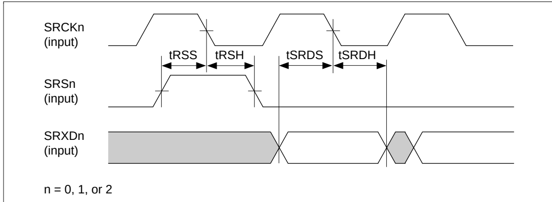
Figure 23.61 SIO Receive Timing
