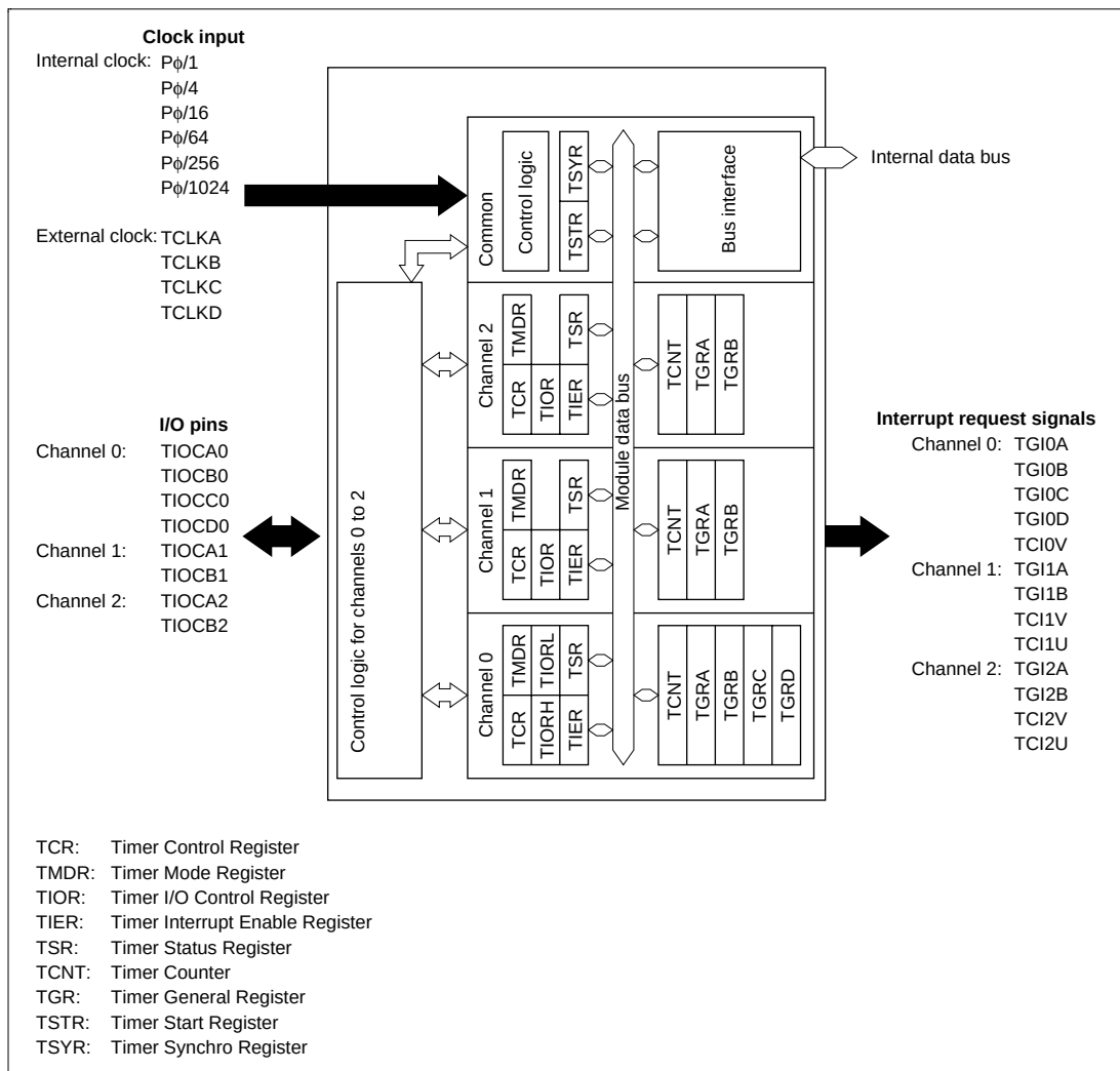
Figure 18.1 TPU Block Diagram
