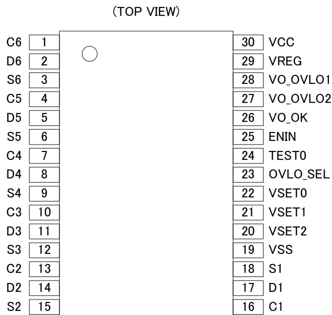
Figure 2 Pin Configuration
