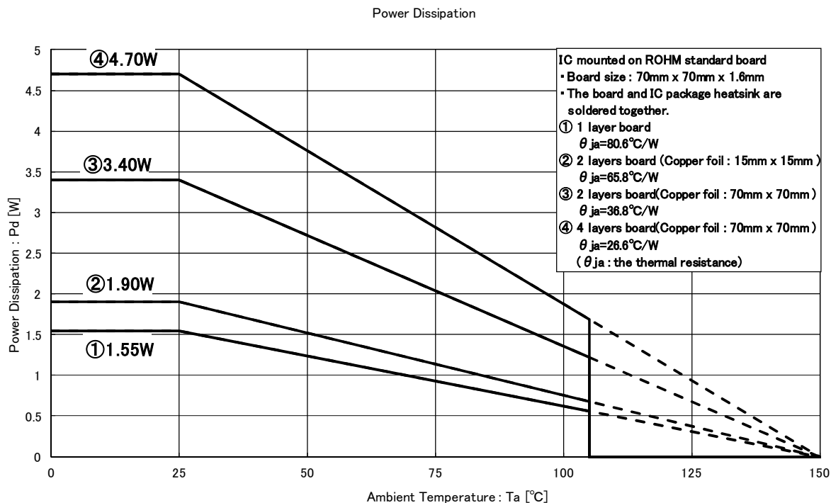
Figure 11. Power Dissipation
