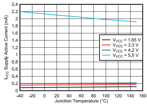
Figure 7-8. Active Current ( I_{VCC} ) vs. Junction Temperature ( T_J )
