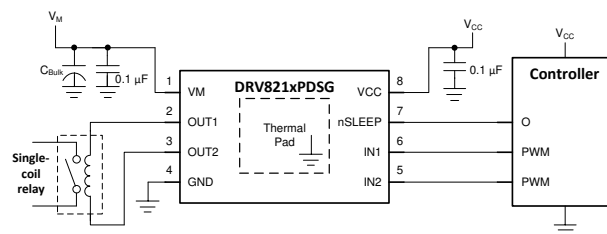
Figure 9-2. PWM interface relay-driving application
