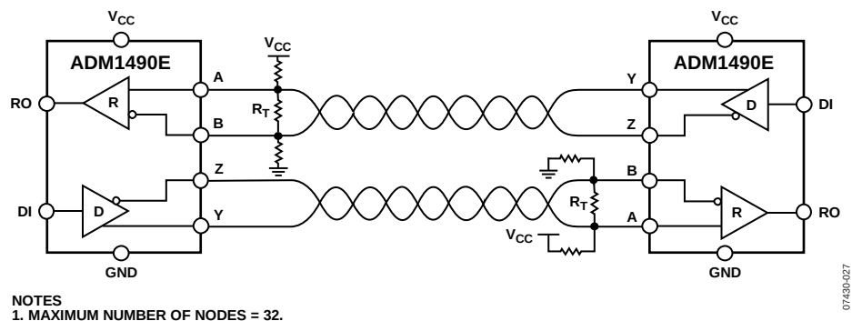
Figure 29. Typical Point-to-Point Full-Duplex Application
