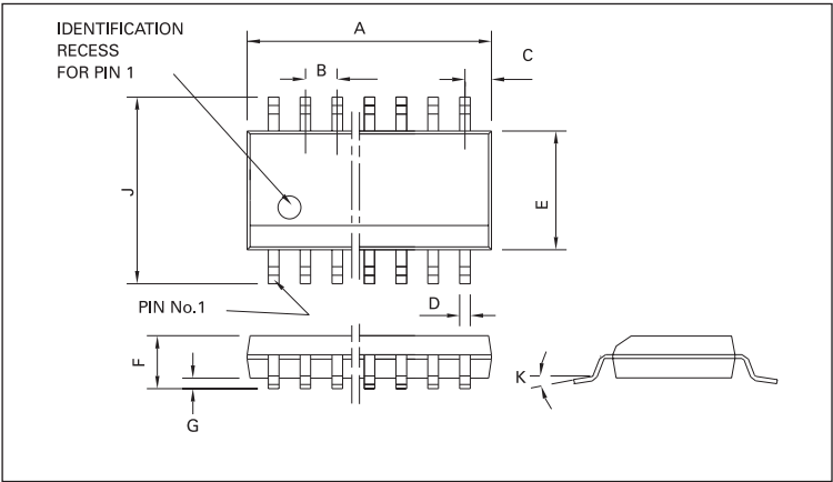
PACKAGE DIMENSIONS
