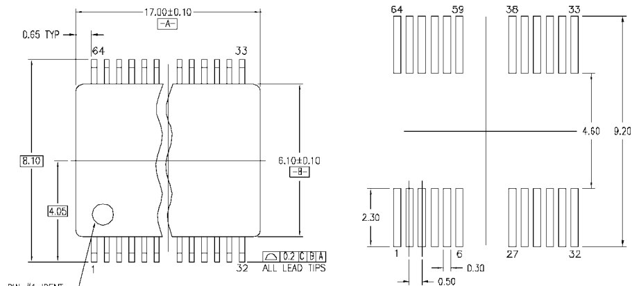
LAND PATTERN RECOMENDATION
