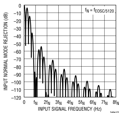
Figure 21. Input Normal Mode Rejection at DC
