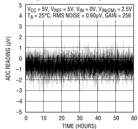
Long-Term ADC Readings
