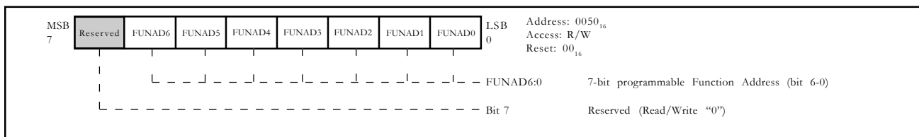
Fig. 1.53. Function Address Register (USBA)
